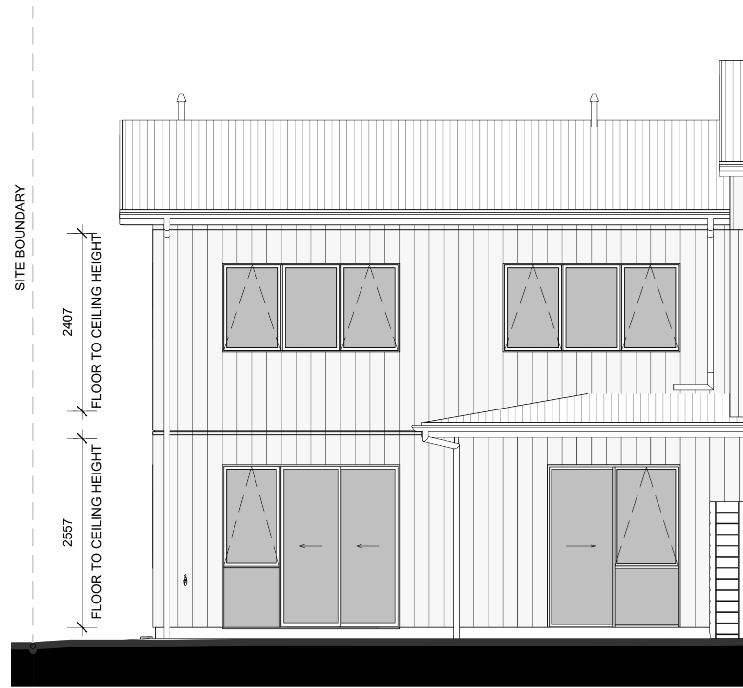
LOT 77 - NORTH ELEVATION
