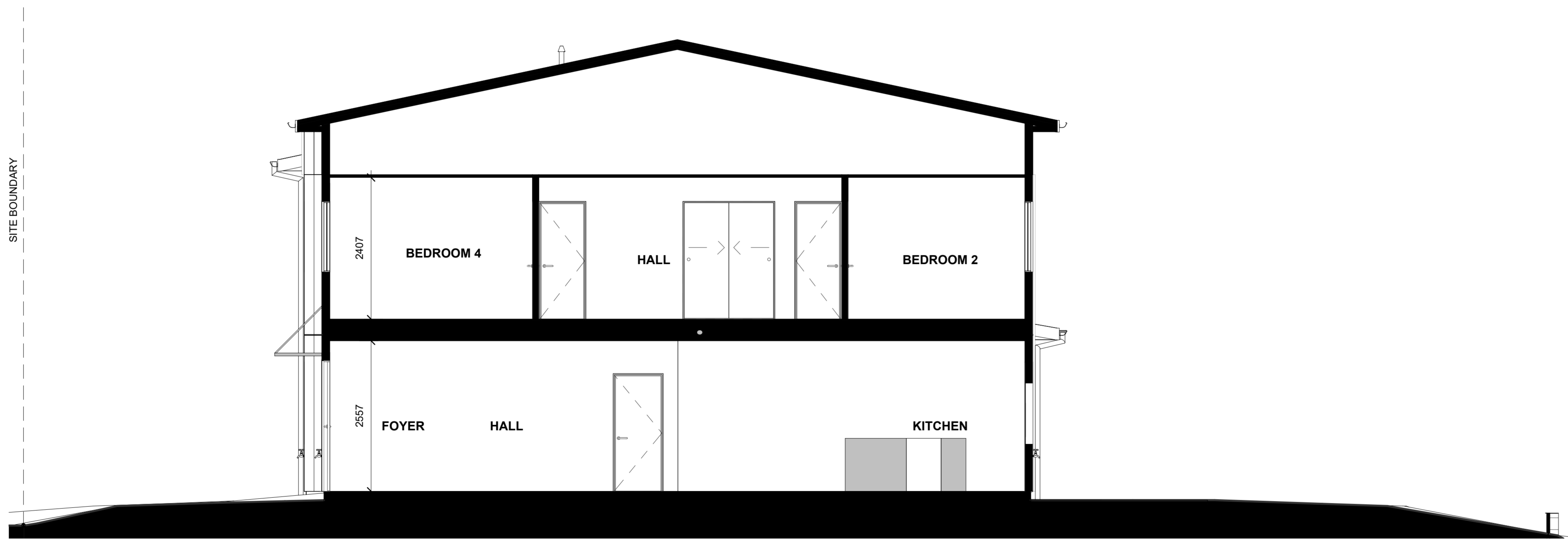
LOT 79 - SECTION A-A
