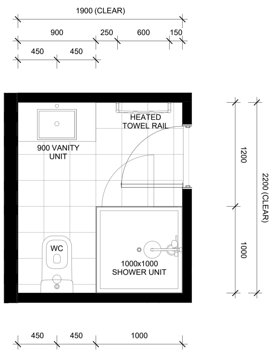
LOT 80 - GROUND FLOOR BATHROOM LAYOUT
