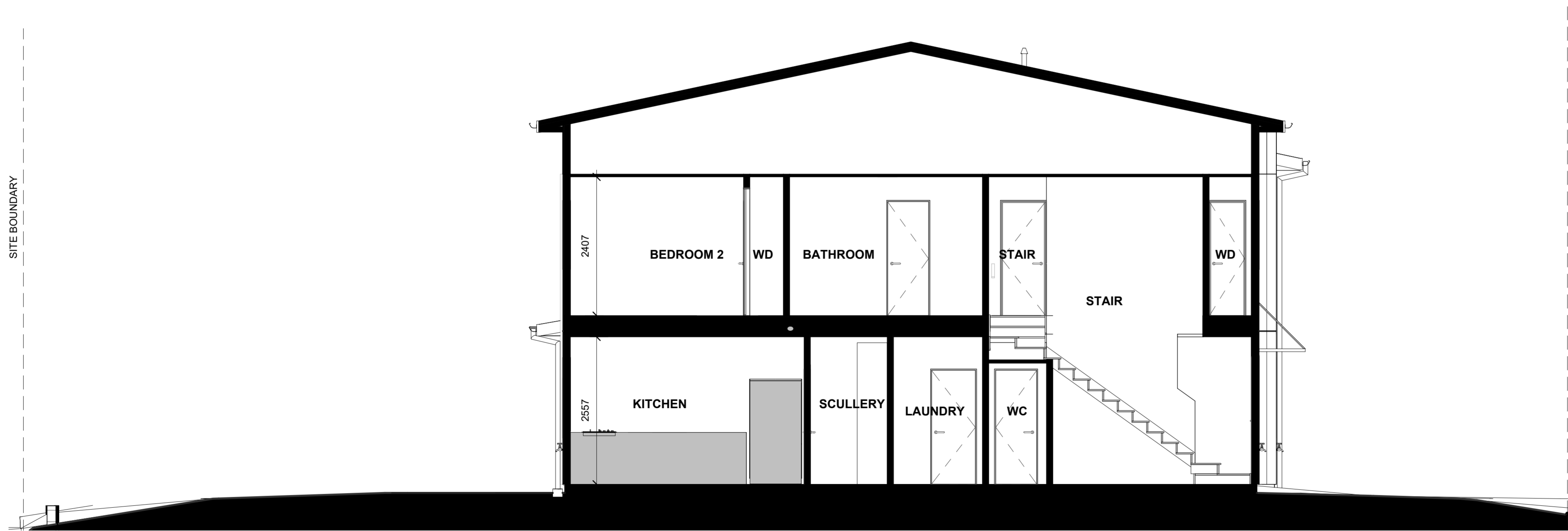
LOT 78 - SECTION A-A
