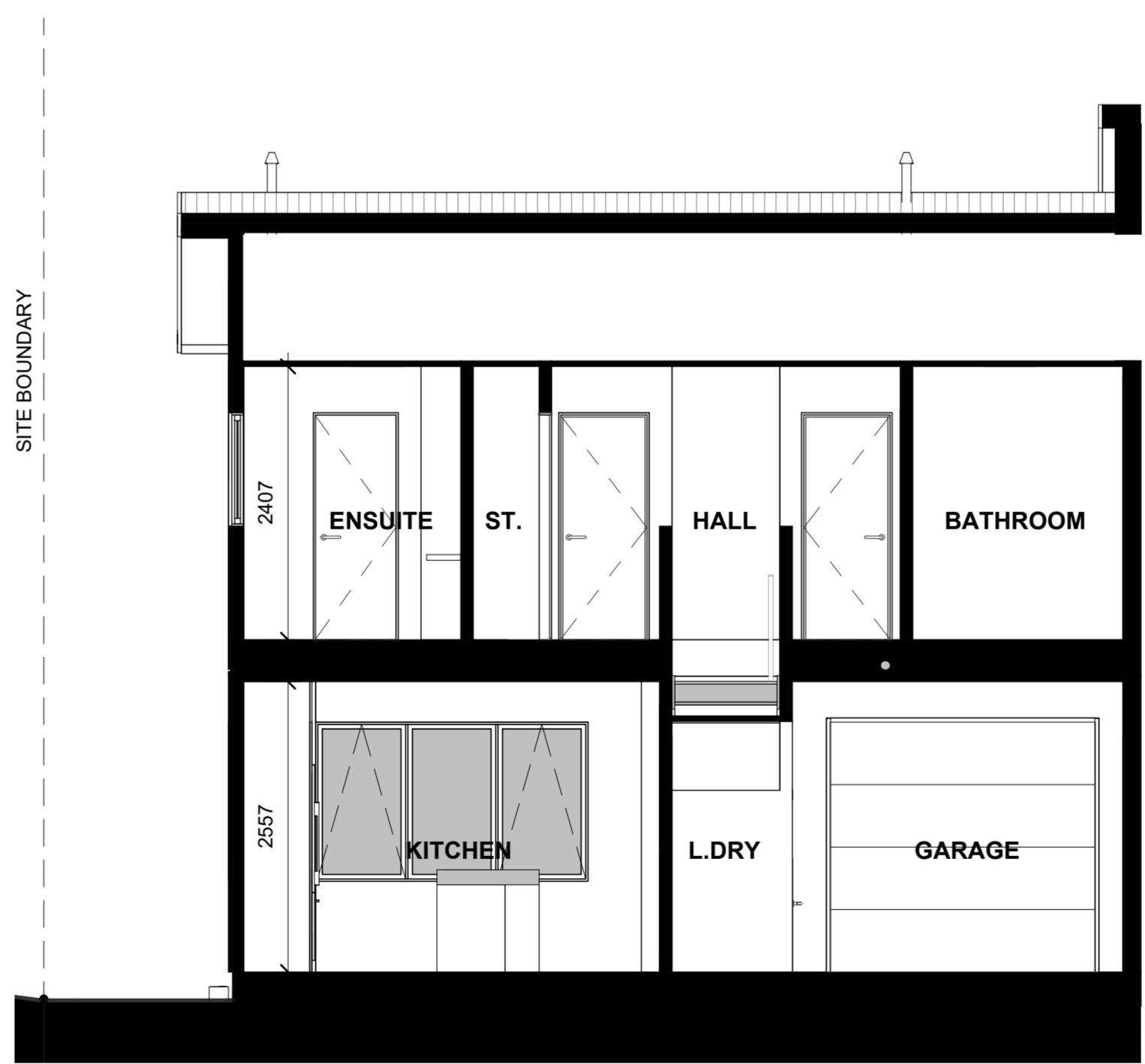
LOT 77 - SECTION B-B
