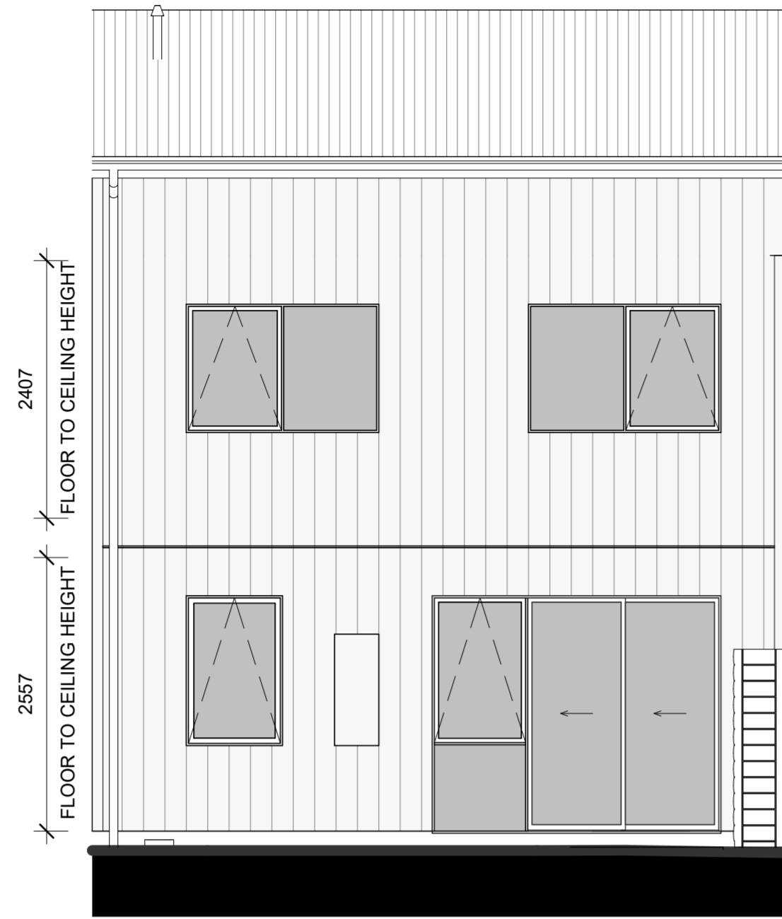
LOT 79 - NORTH ELEVATION
