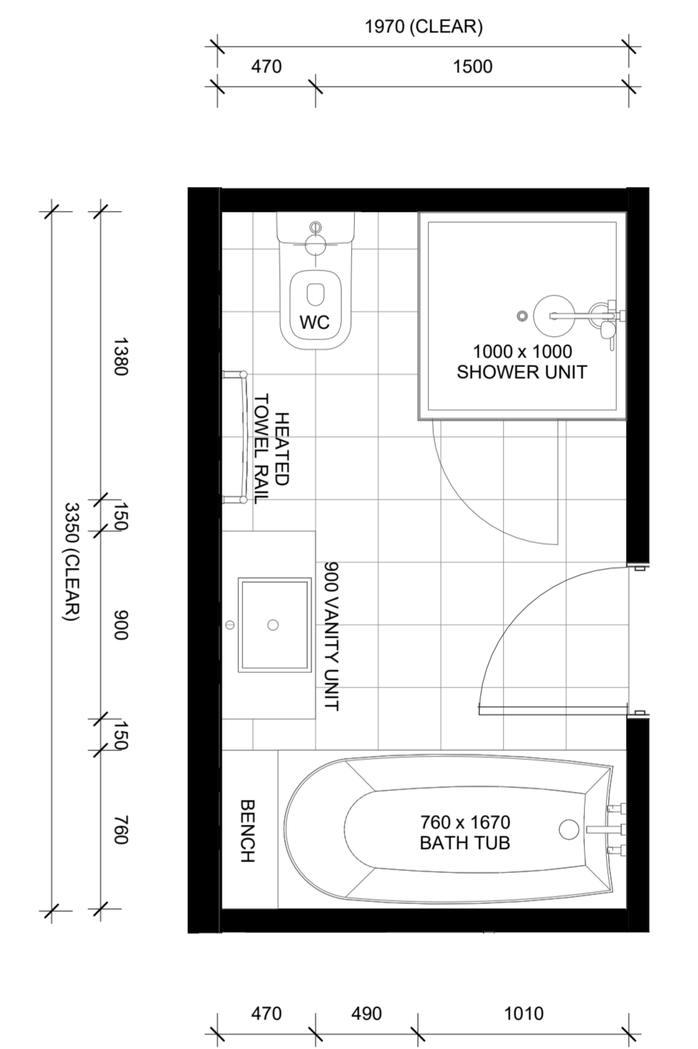
LOT 78 - FIRST FLOOR BATHROOM LAYOUT
