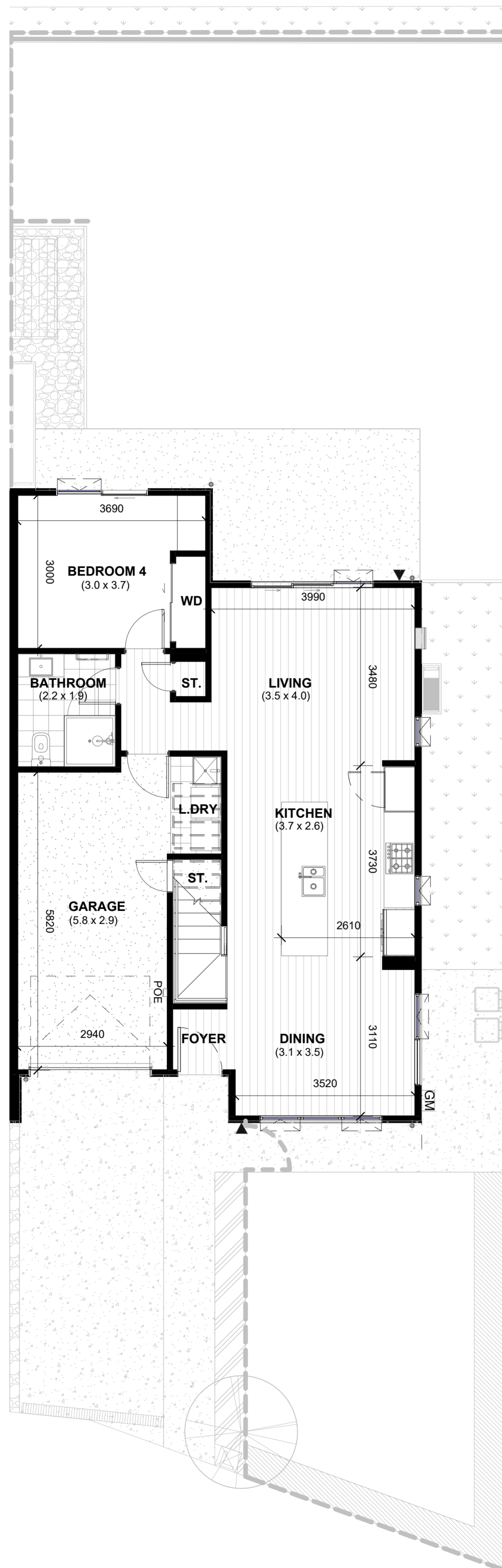
LOT 77 - GROUND FLOOR DIMENSION PLAN
