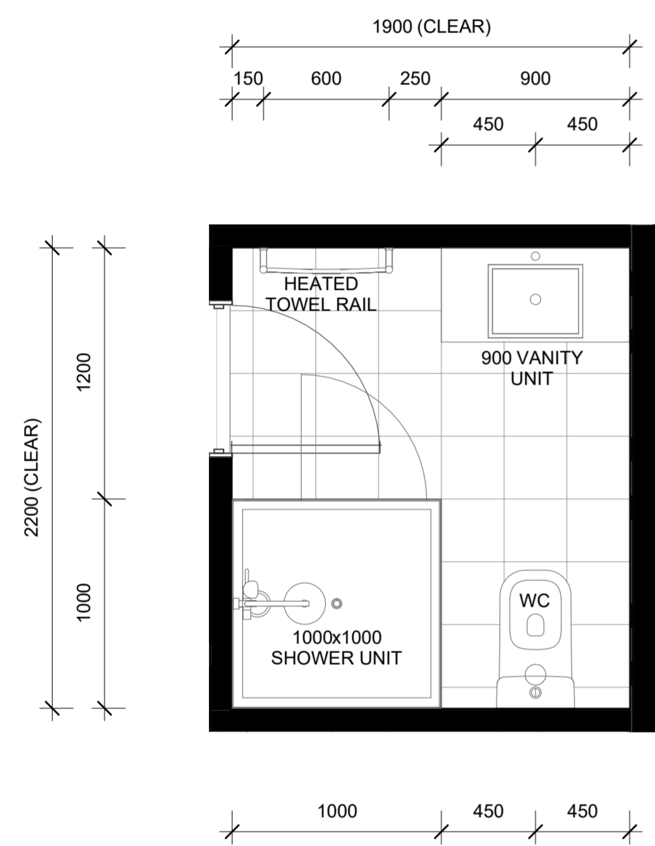
LOT 77 - GROUND FLOOR BATHROOM LAYOUT
