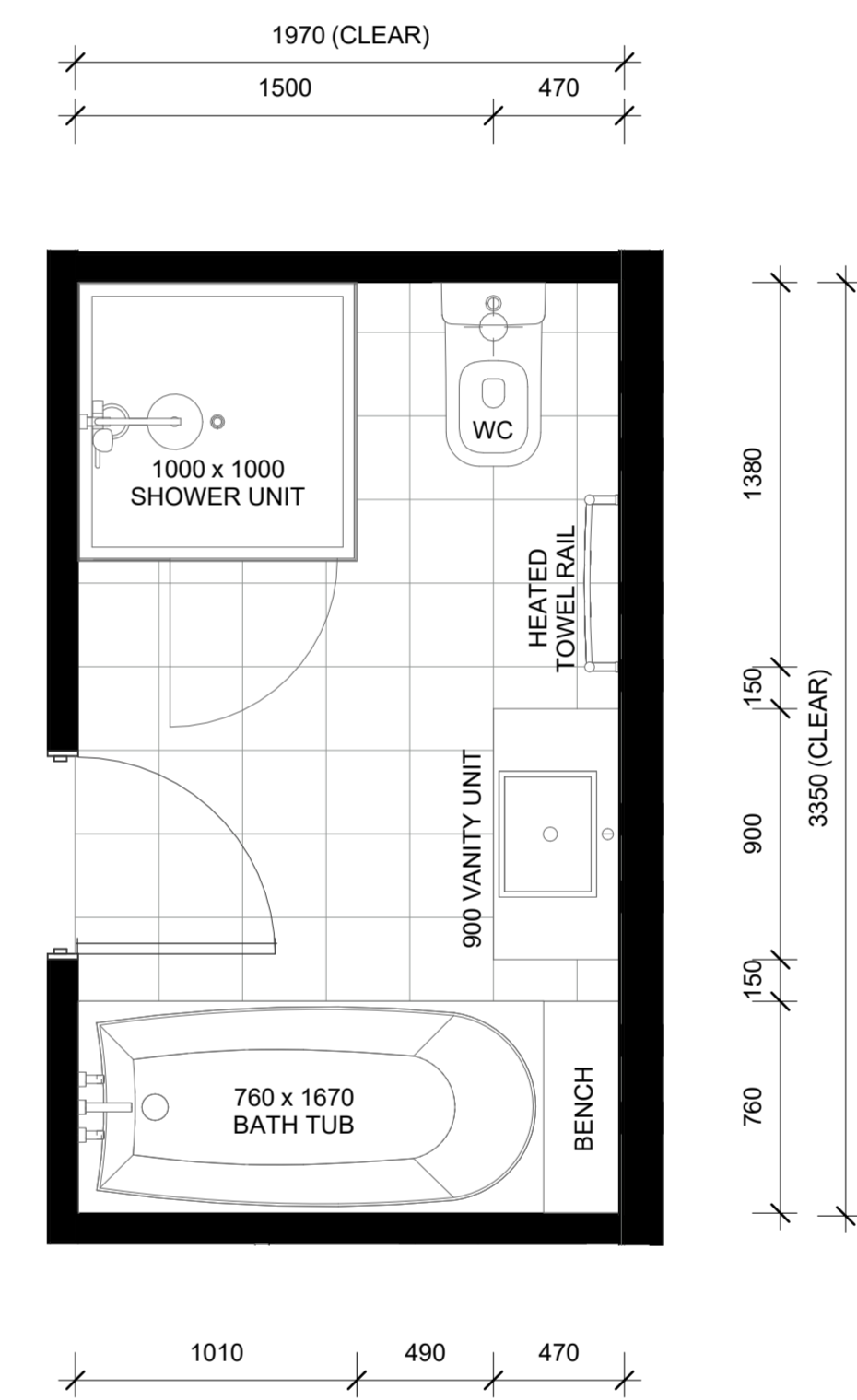
LOT 79 - FIRST FLOOR BATHROOM LAYOUT
