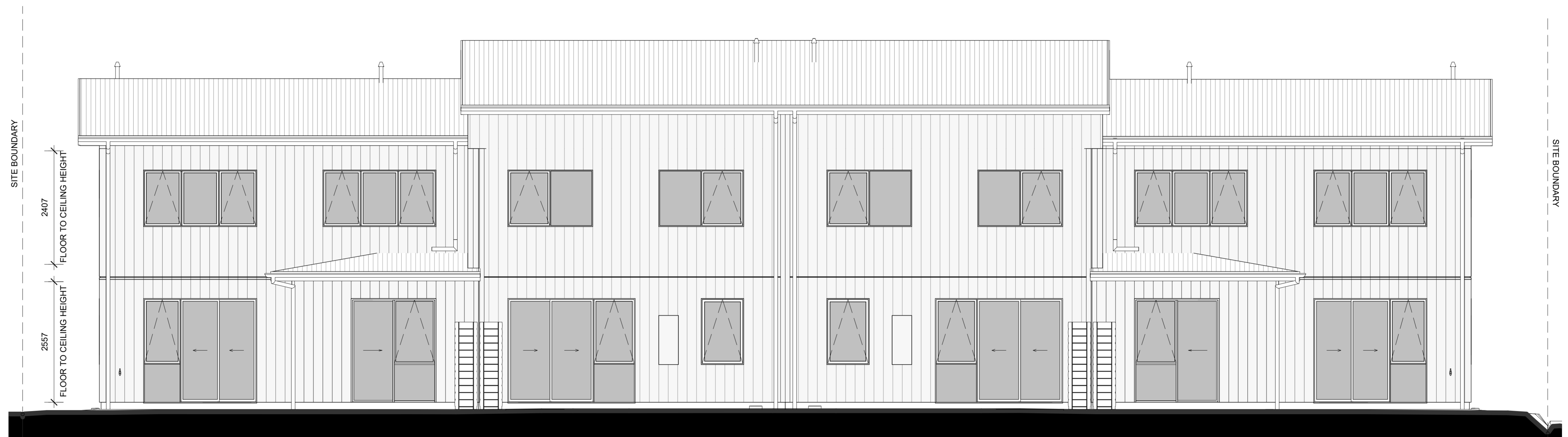
OVERALL NORTH ELEVATION
