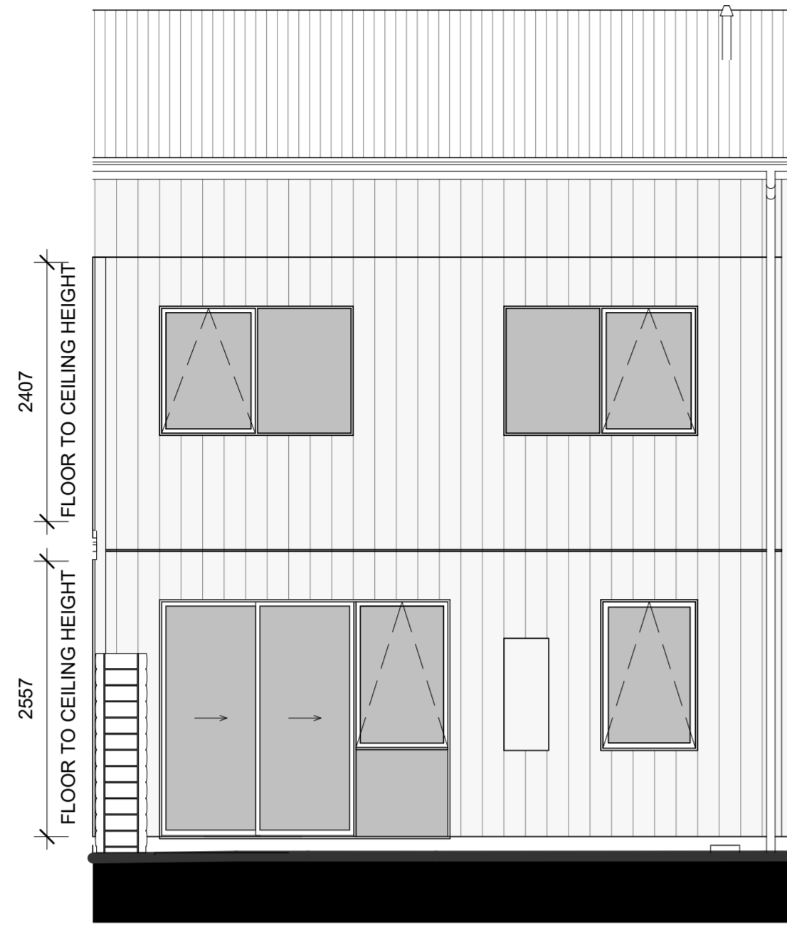
LOT 78 - NORTH ELEVATION
