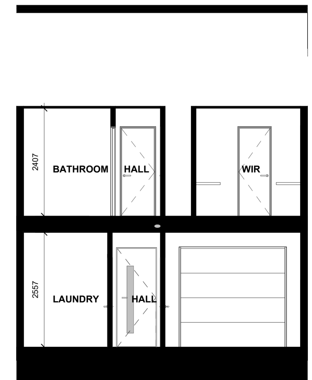
LOT 79 - SECTION B-B
