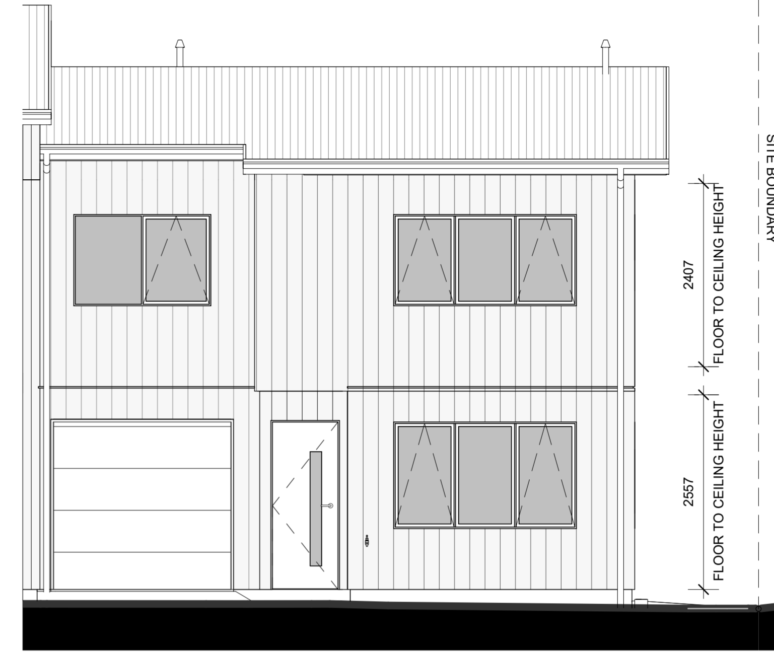
LOT 77 - SOUTH ELEVATION
