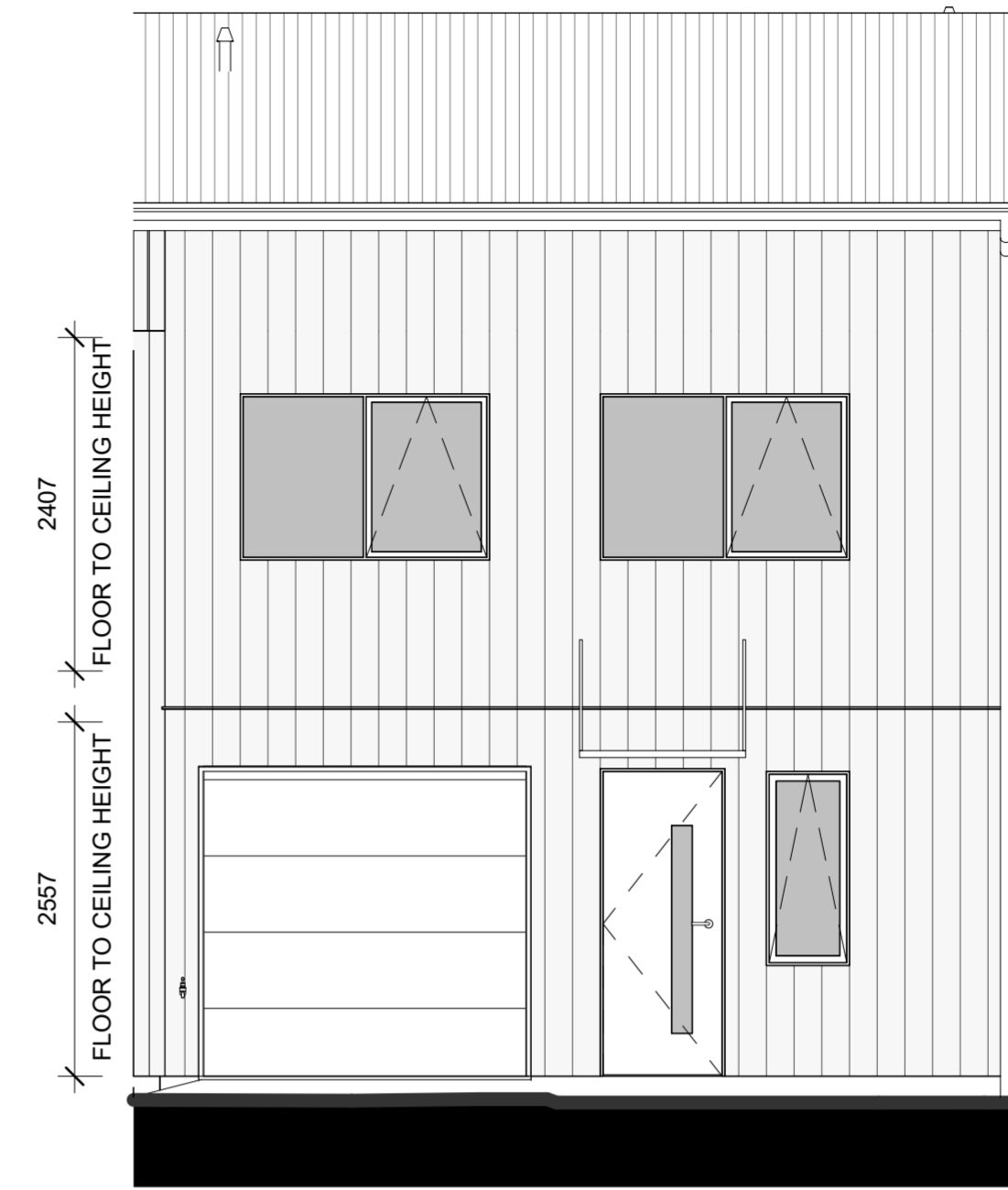
LOT 79 - SOUTH ELEVATION
