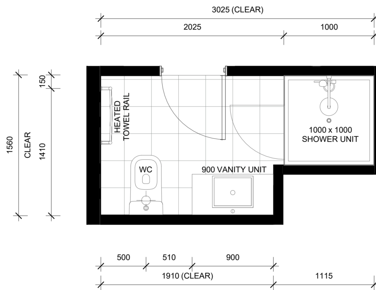
LOT 79 - FIRST FLOOR ENSUITE LAYOUT
