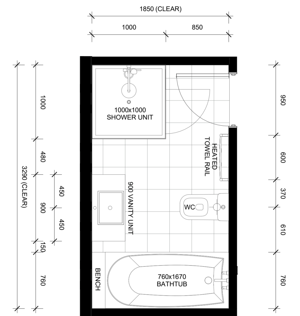
LOT 80 - FIRST FLOOR BATHROOM LAYOUT
