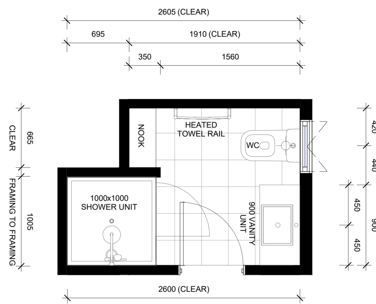
LOT 80 - FIRST FLOOR ENSUITE PLAN
