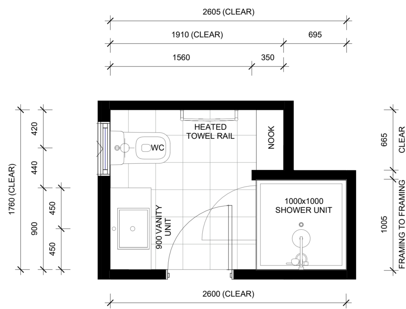
LOT 77 - FIRST FLOOR ENSUITE PLAN
