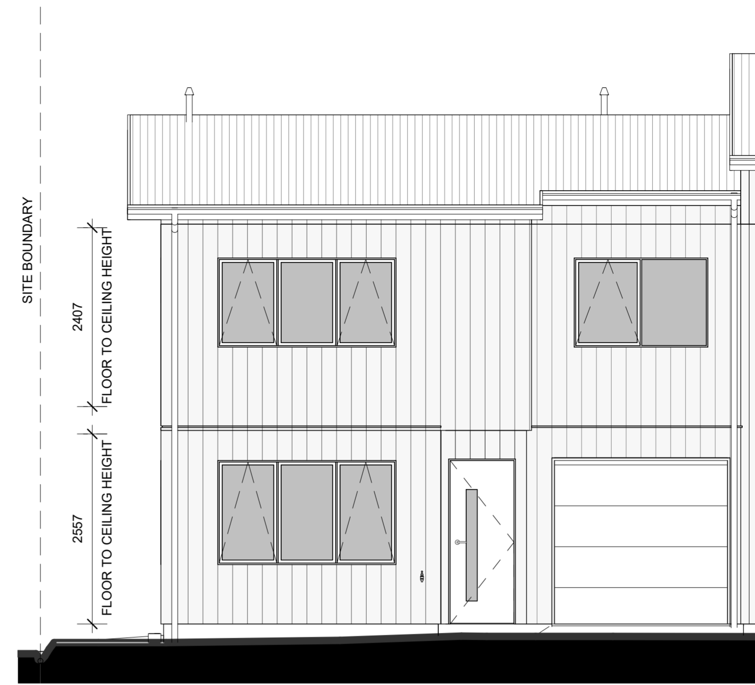
LOT 80 - SOUTH ELEVATION
