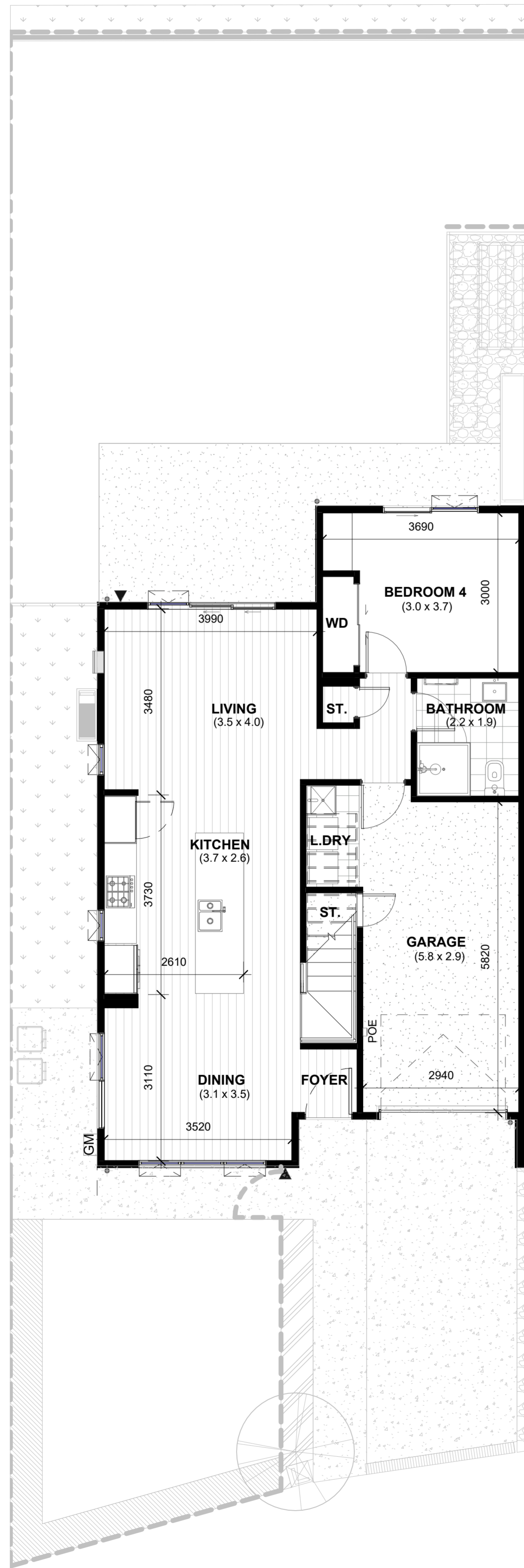
LOT 80 - GROUND FLOOR DIMENSION PLAN
