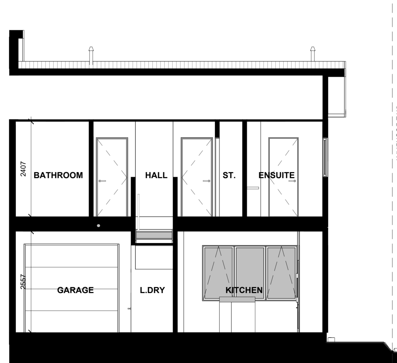
LOT 80 - SECTION B-B
