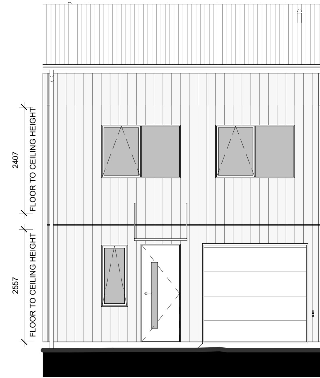
LOT 78 - SOUTH ELEVATION
