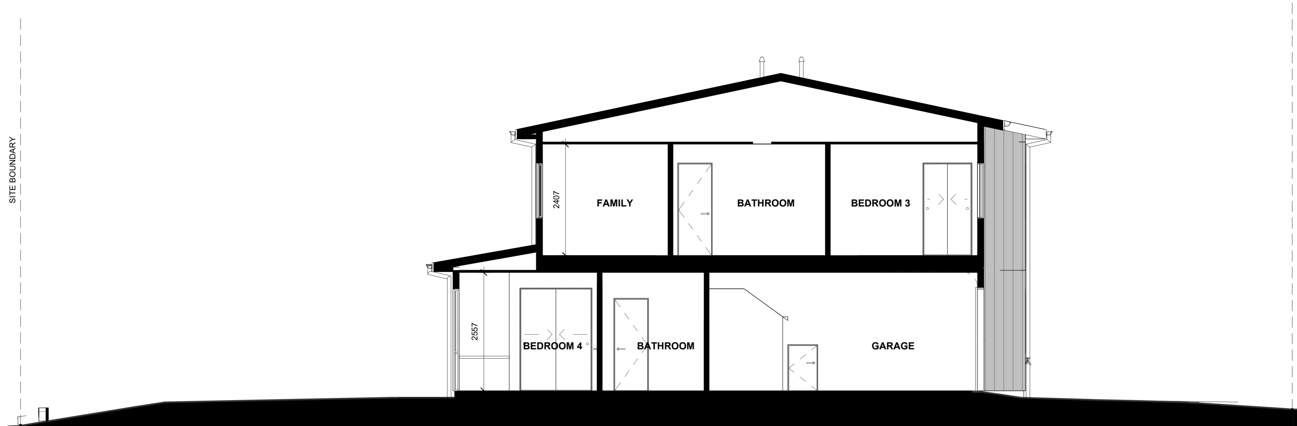
LOT 77 - SECTION A-A
