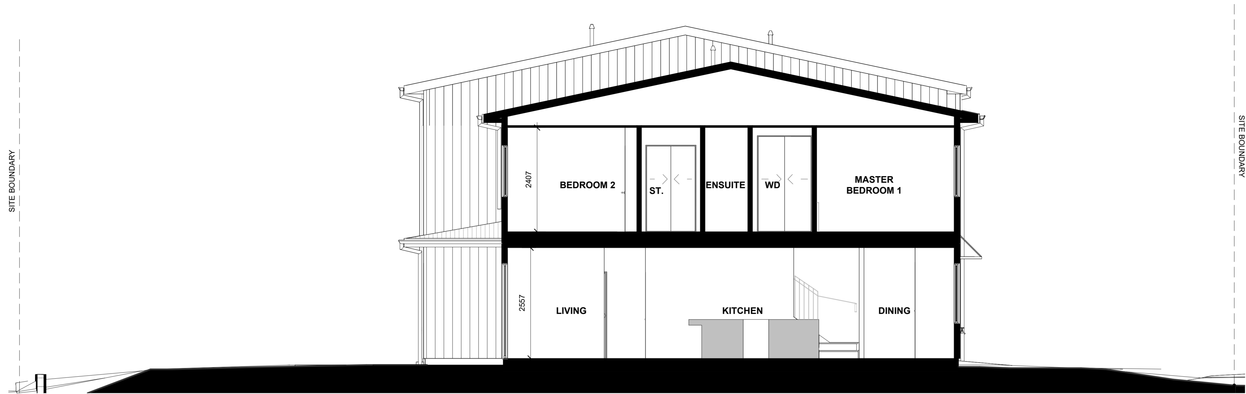
LOT 80 - SECTION A-A
