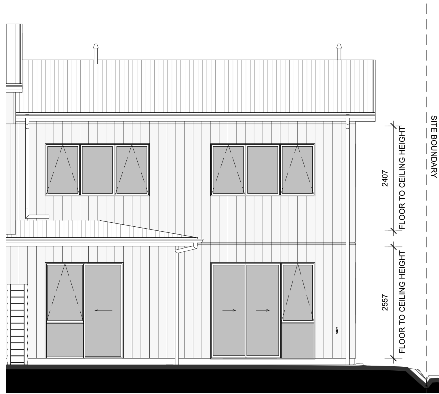
LOT 80 - NORTH ELEVATION
