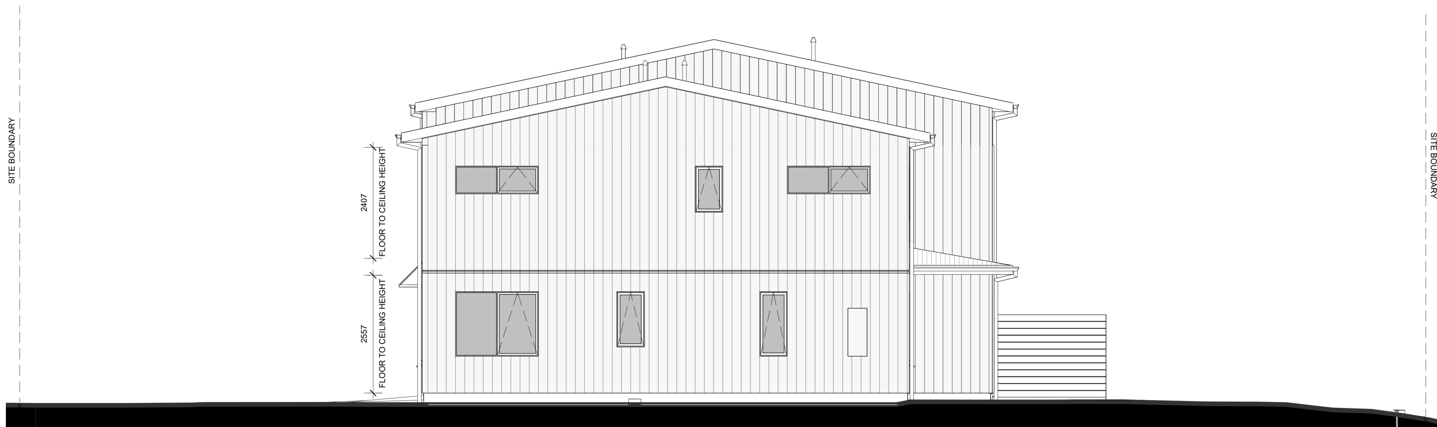
LOT 77 - EAST ELEVATION
