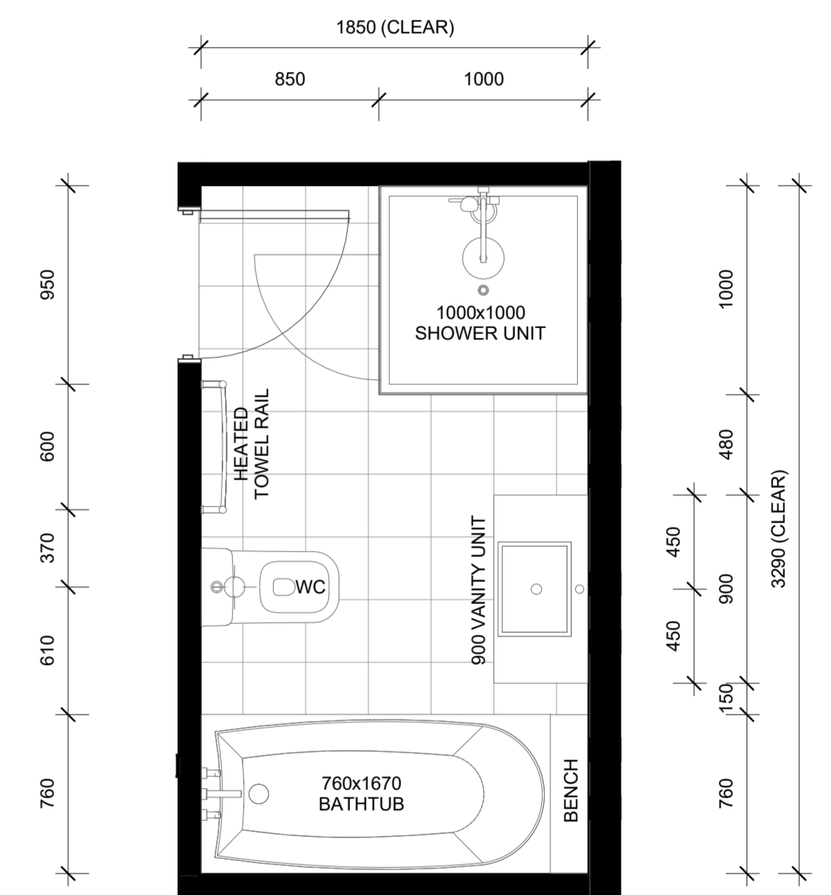
LOT 77 - FIRST FLOOR BATHROOM LAYOUT
