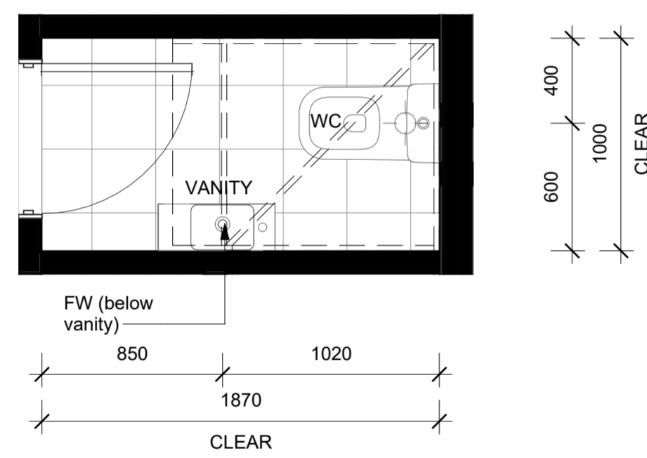
LOT 79 - GROUND FLOOR WC LAYOUT
