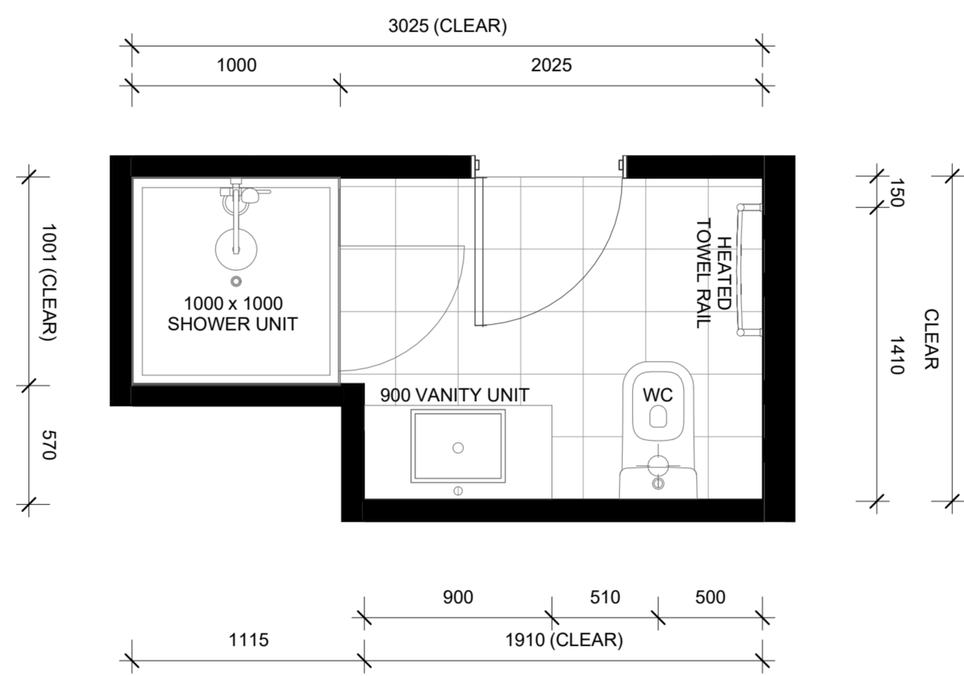
LOT 78 - FIRST FLOOR ENSUITE LAYOUT
