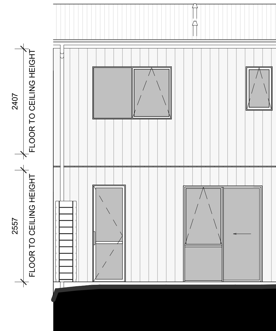
LOT 122 - WEST ELEVATION
