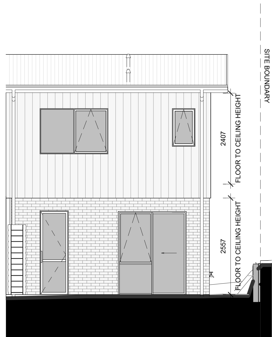
LOT 121 - WEST ELEVATION
