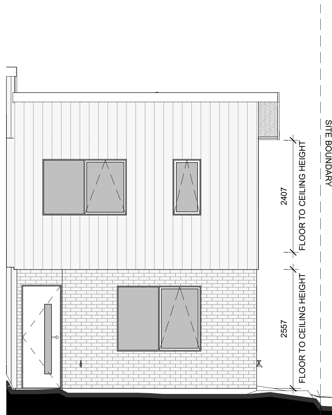
LOT 123 - EAST ELEVATION
