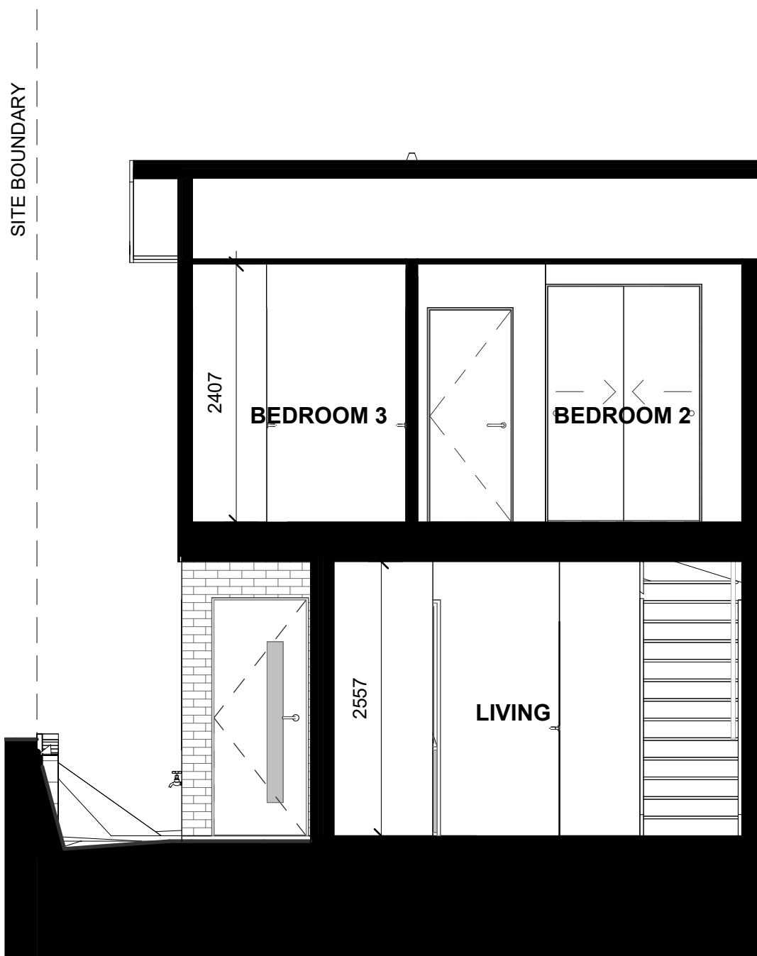
LOT 121 - SECTION B-B
