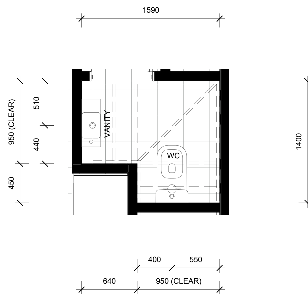
LOT 123 - GROUND FLOOR WC LAYOUT
