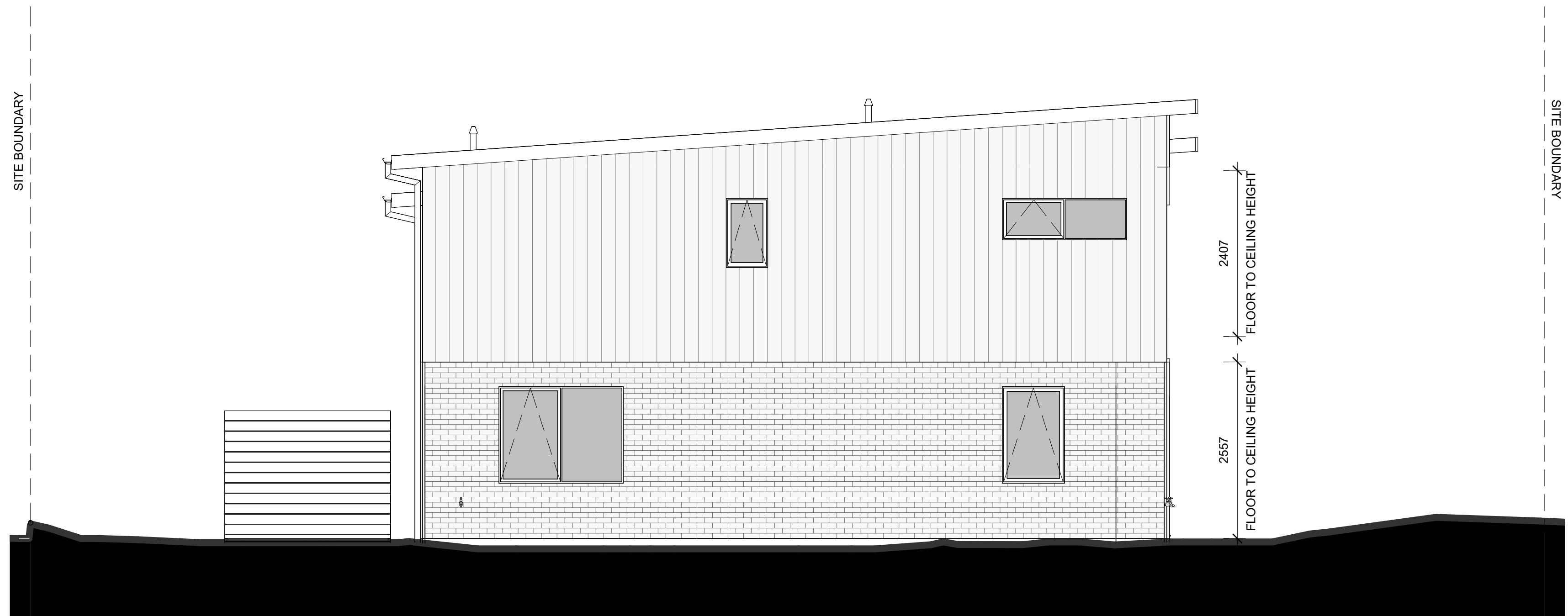
LOT 121 - SOUTH ELEVATION
