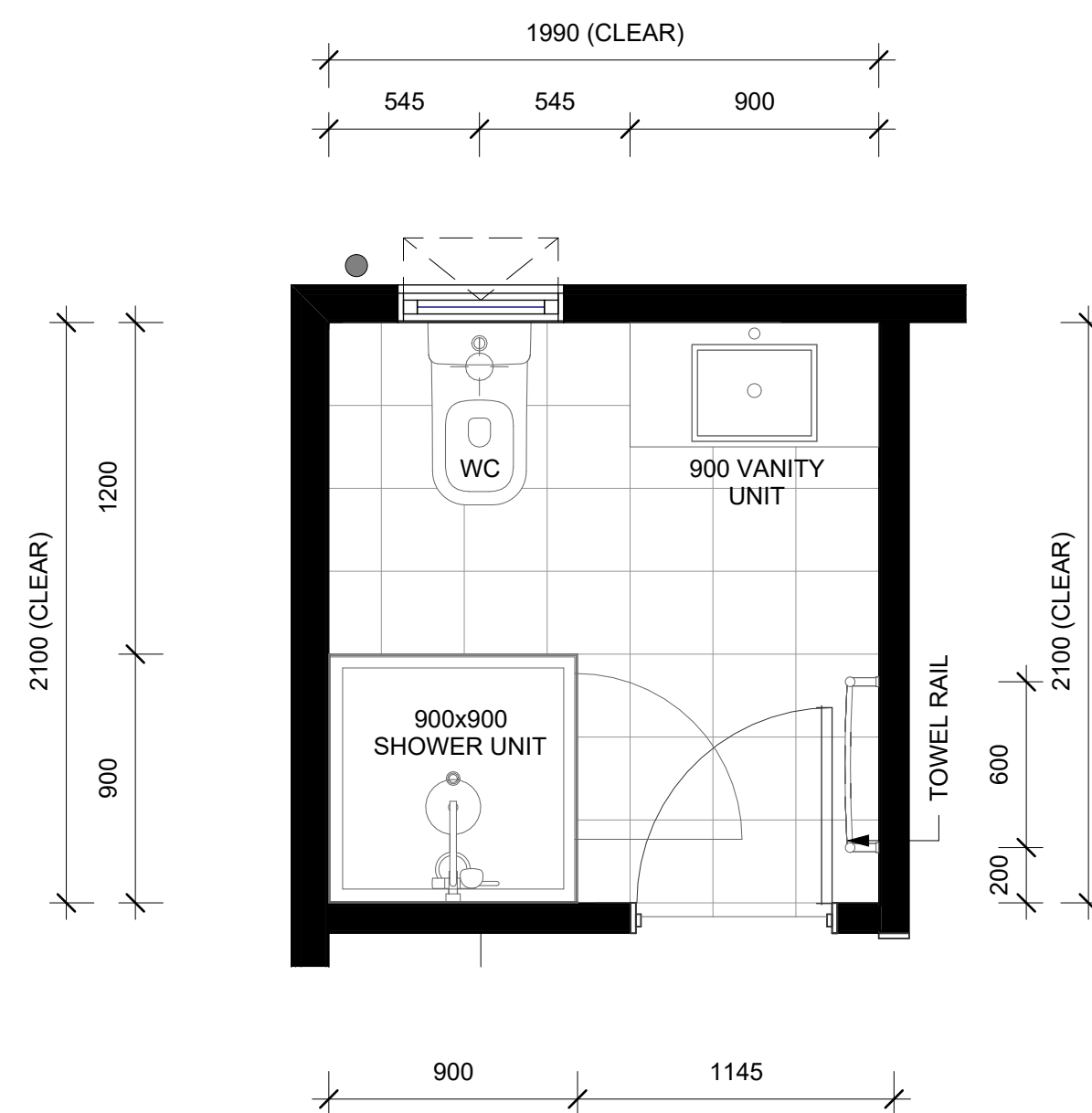
LOT 123 - FIRST FLOOR ENSUITE LAYOUT
