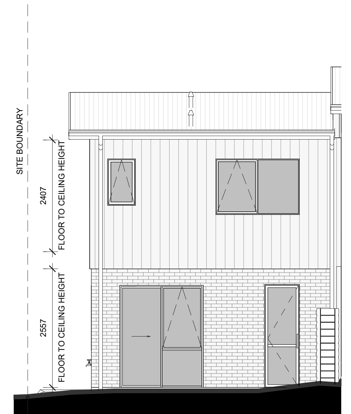
LOT 123 - WEST ELEVATION
