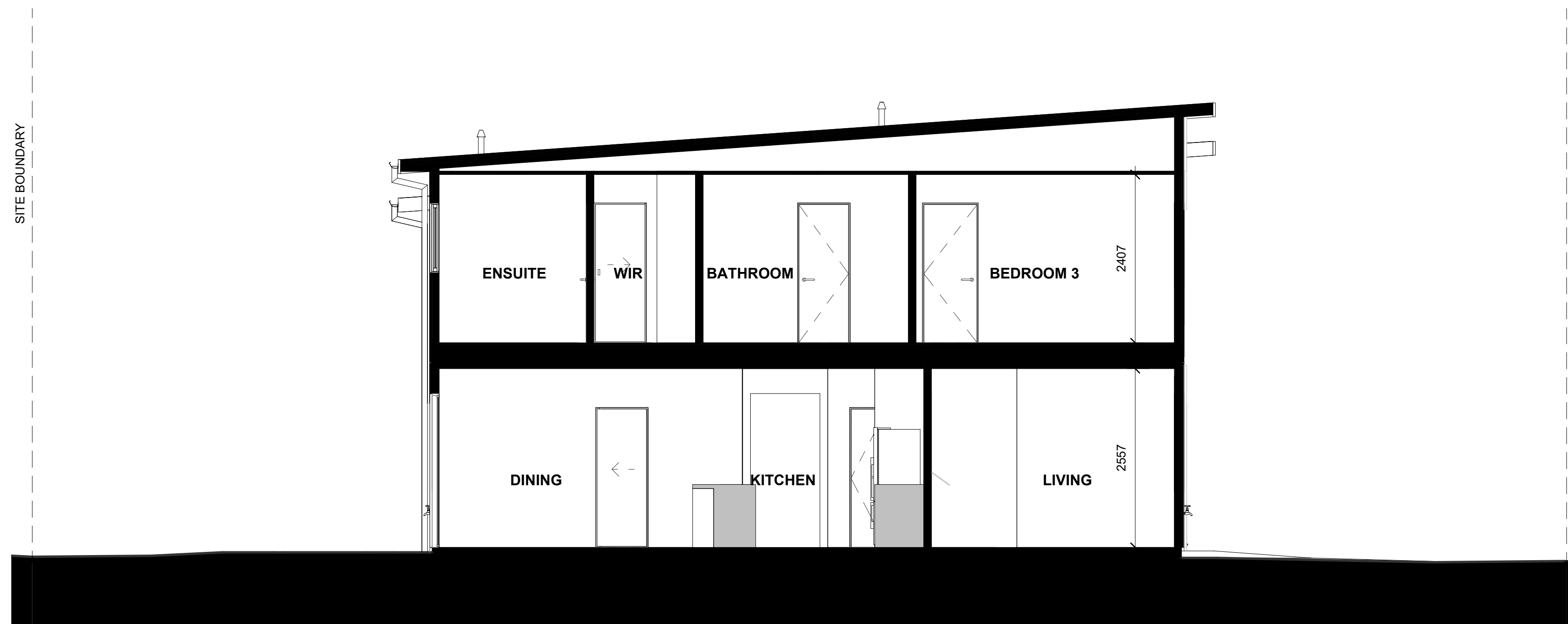
LOT 122 - SECTION A-A
