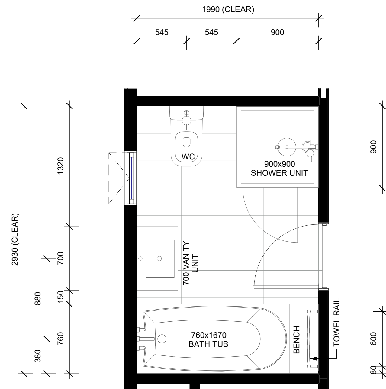
LOT 123 - FIRST FLOOR BATHROOM LAYOUT
