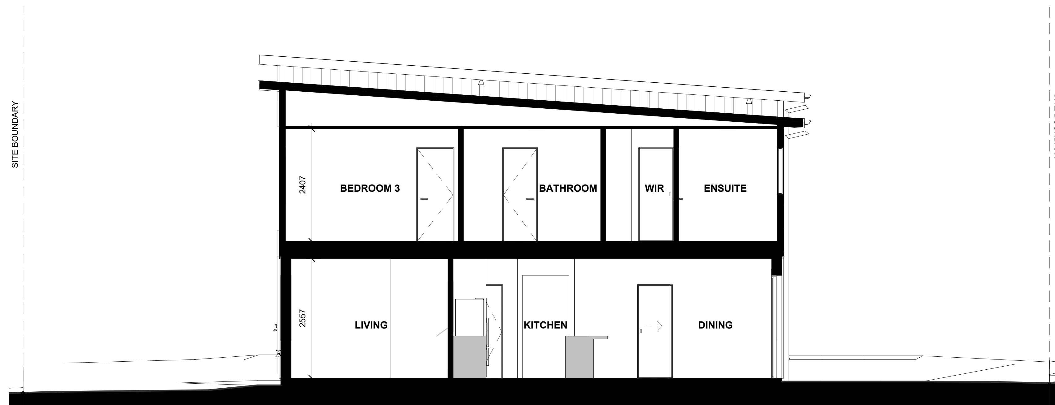
LOT 123 - SECTION A-A
