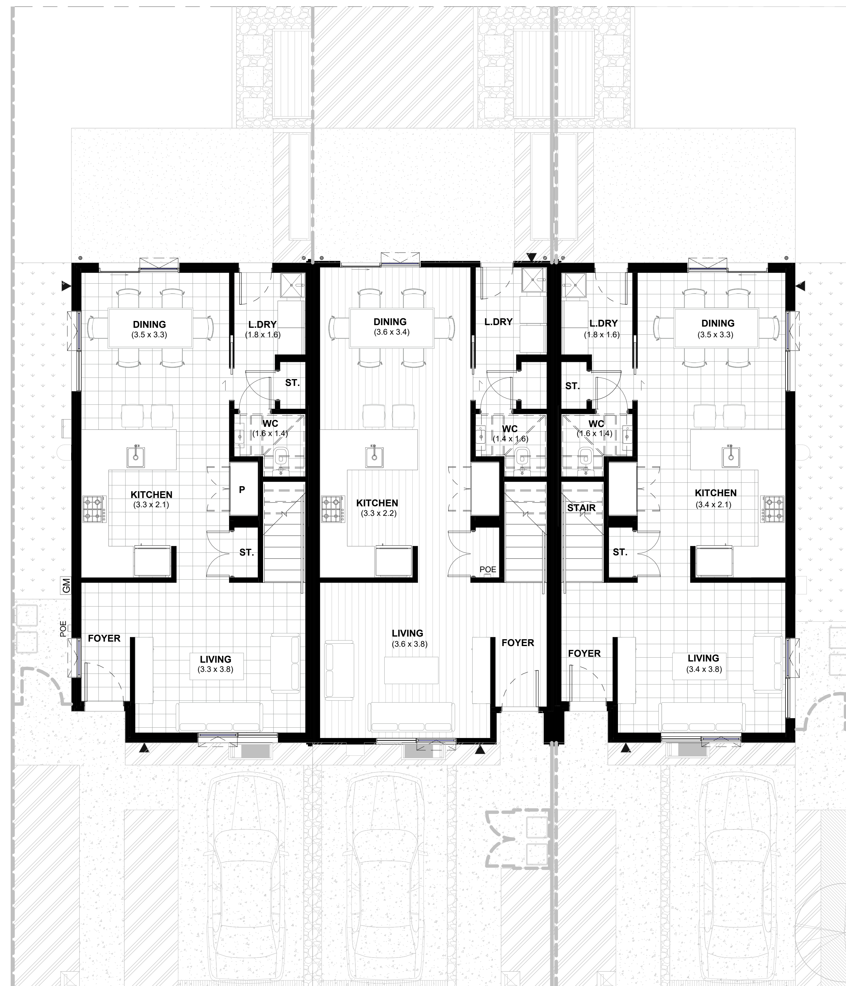
LOT 121 GROUND FLOOR PLAN 13 NUKU PLACE, MANUREWA Floor Area - 114m 2 Site Area - 147m 2
