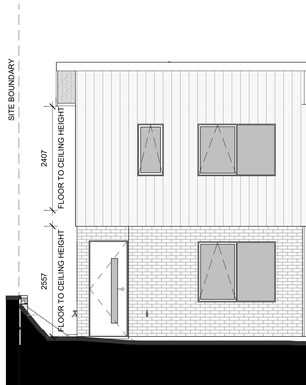
LOT 121 - EAST ELEVATION
