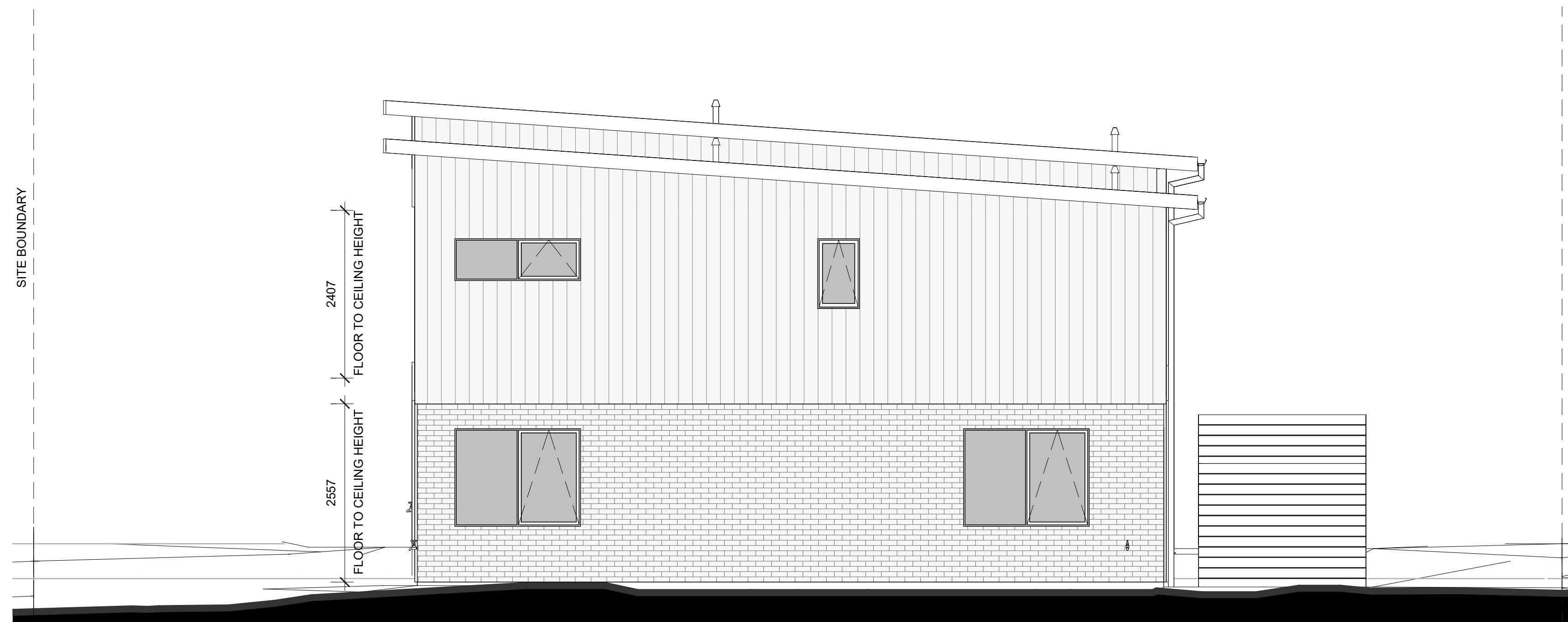
LOT 123 - NORTH ELEVATION
