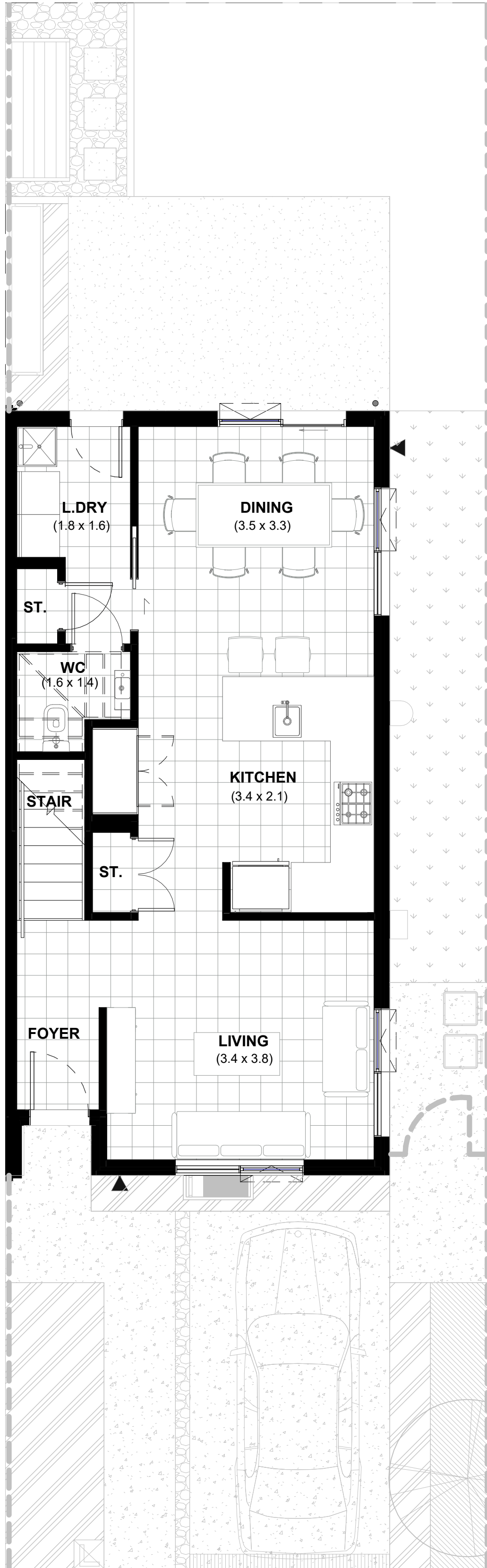
LOT 123 - GROUND FLOOR PLAN
