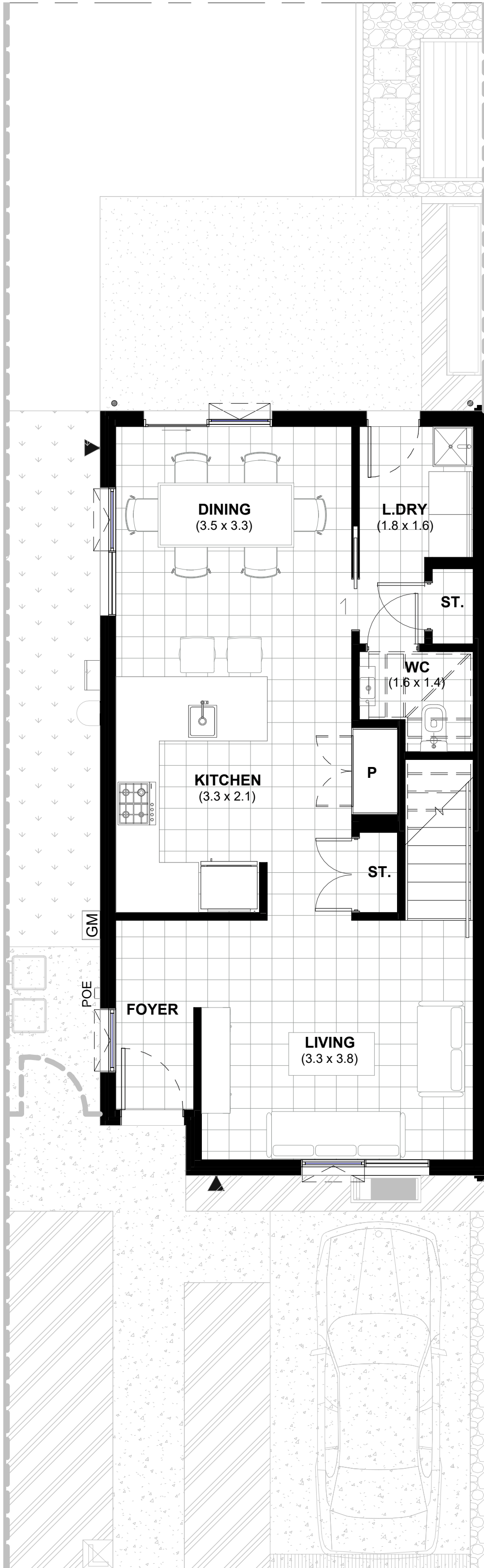
LOT 121 - GROUND FLOOR PLAN
