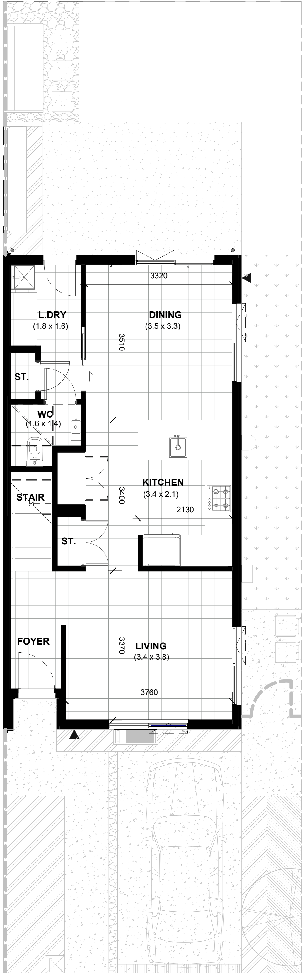
LOT 123 - GROUND FLOOR DIMENSION PLAN
