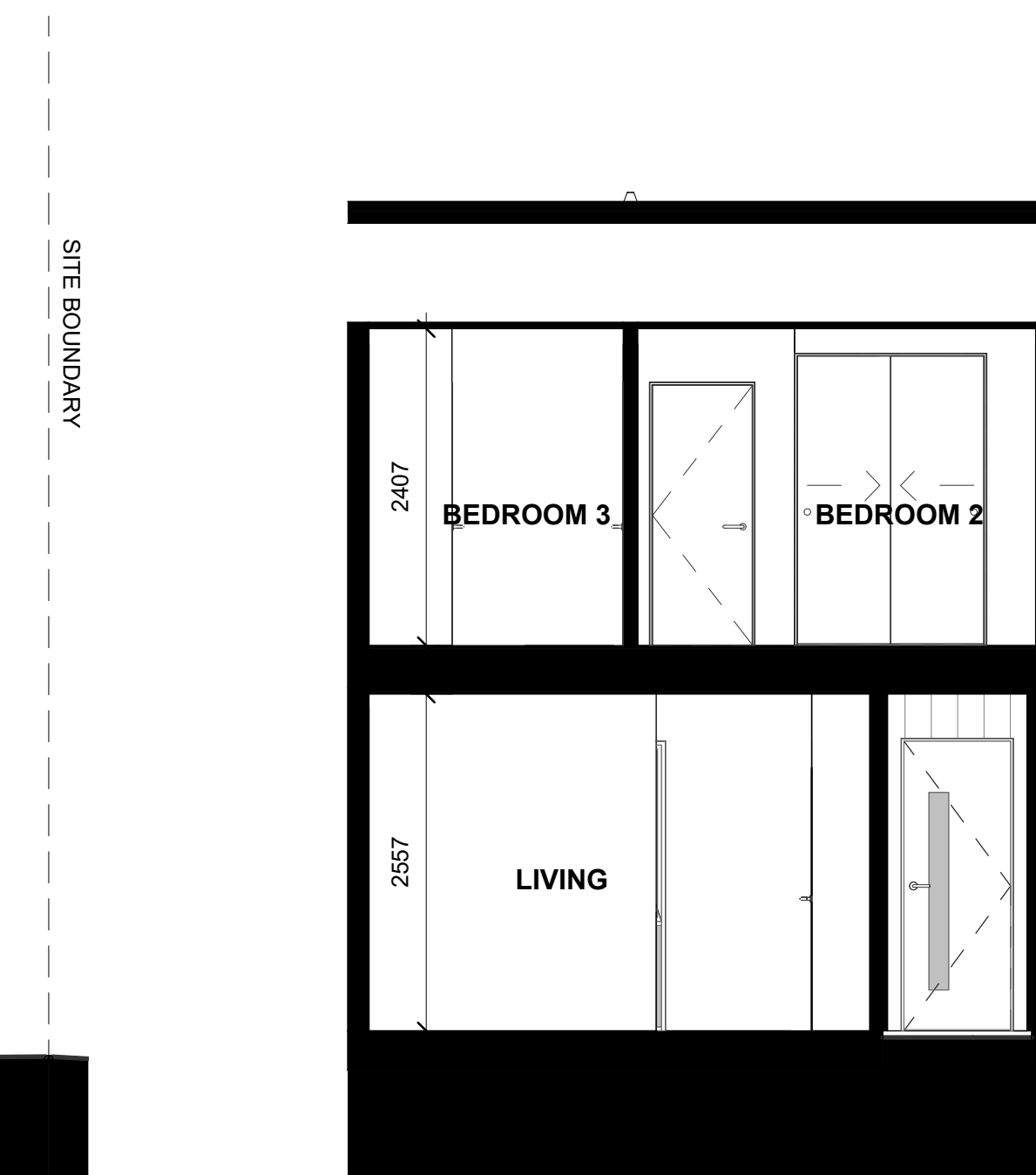
LOT 122 - SECTION B-B
