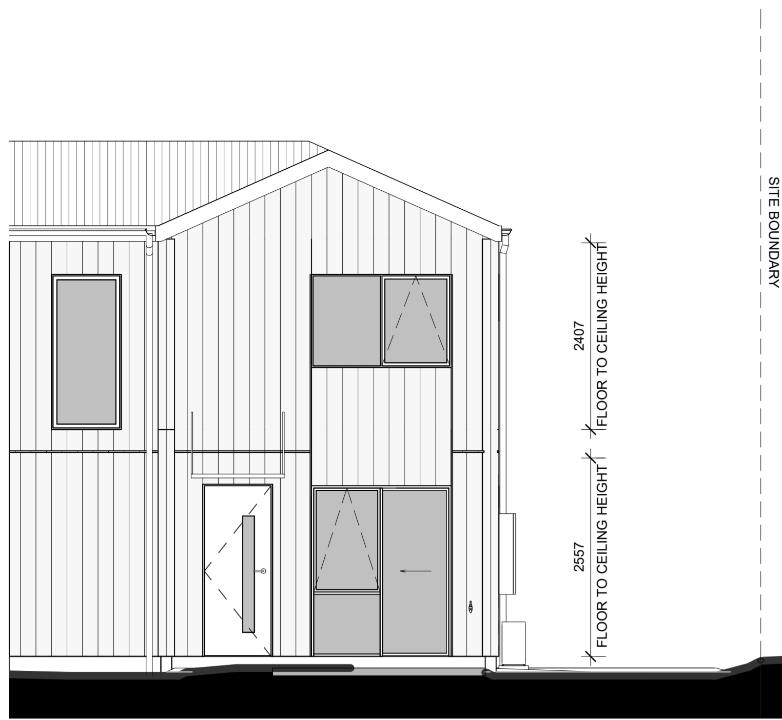
LOT 101 - SOUTH ELEVATION
