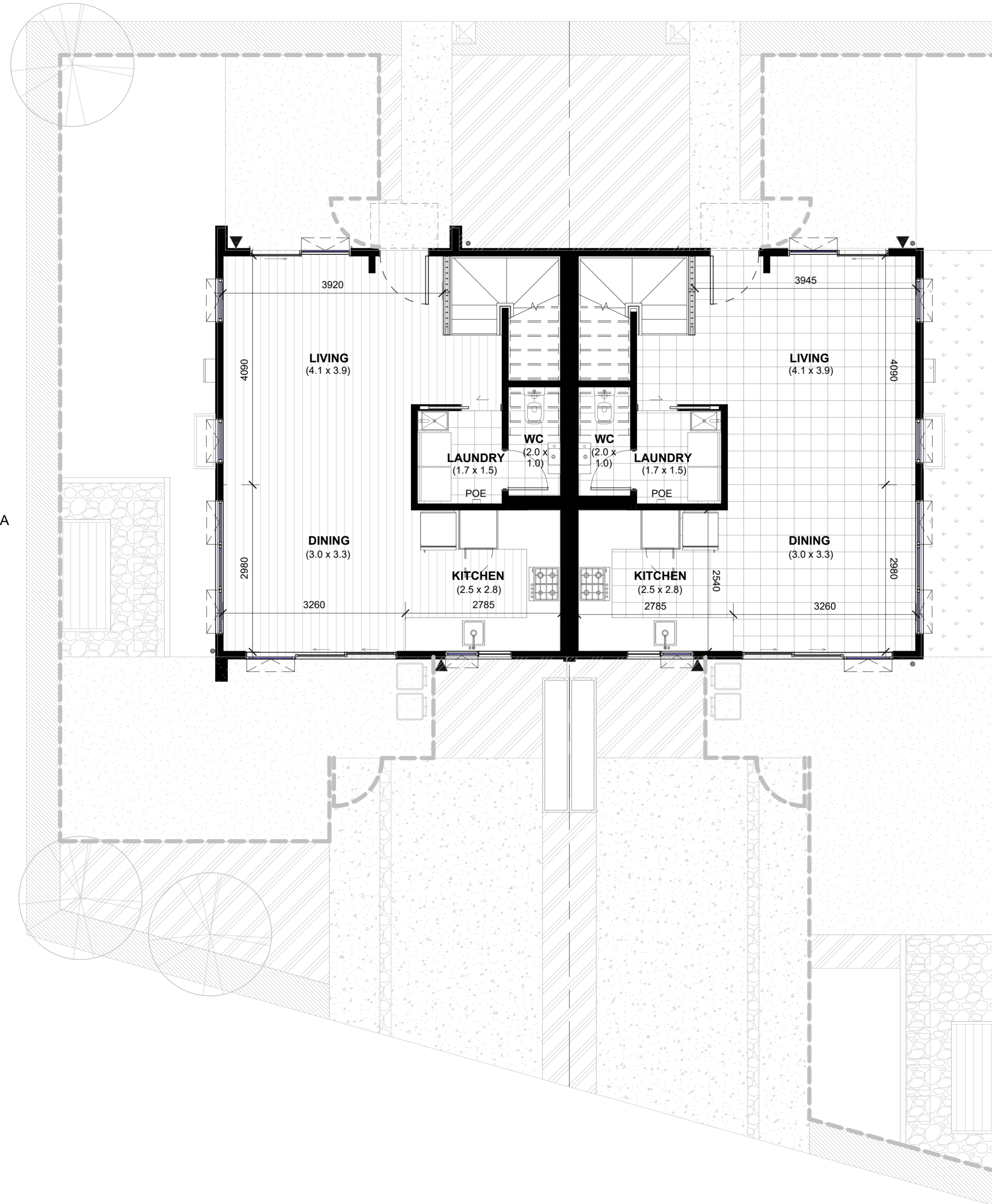
LOT 100 GROUND FLOOR PLAN 3 TARA LANE, MANUREWA Floor Area - 90m 2 Site Area - 155m 2 Ground Floor - 45m 2 First Floor - 45m 2
