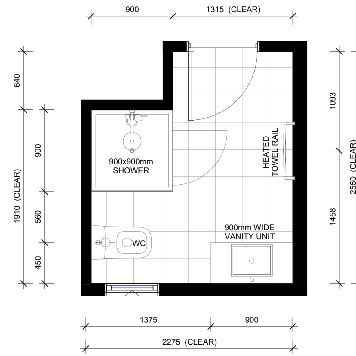
LOT 101 - FIRST FLOOR BATHROOM LAYOUT
