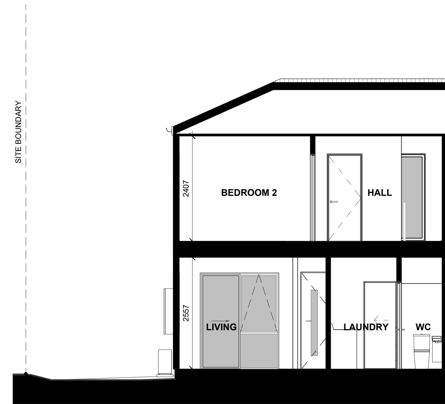
LOT 101 - SECTION B-B
