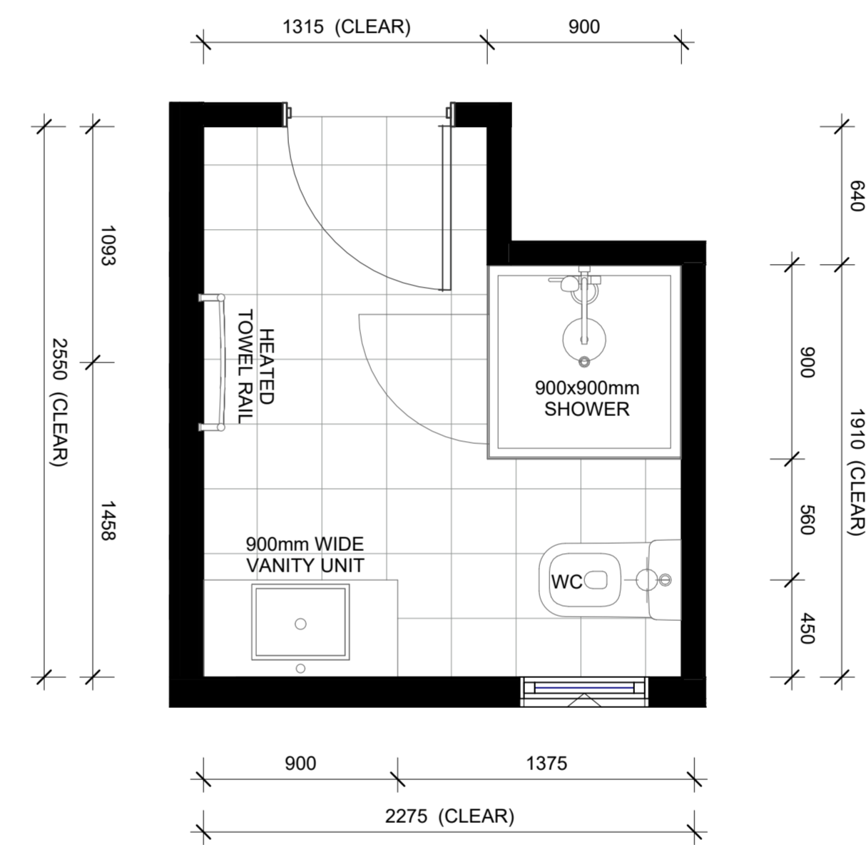
LOT 100 - FIRST FLOOR BATHROOM LAYOUT
