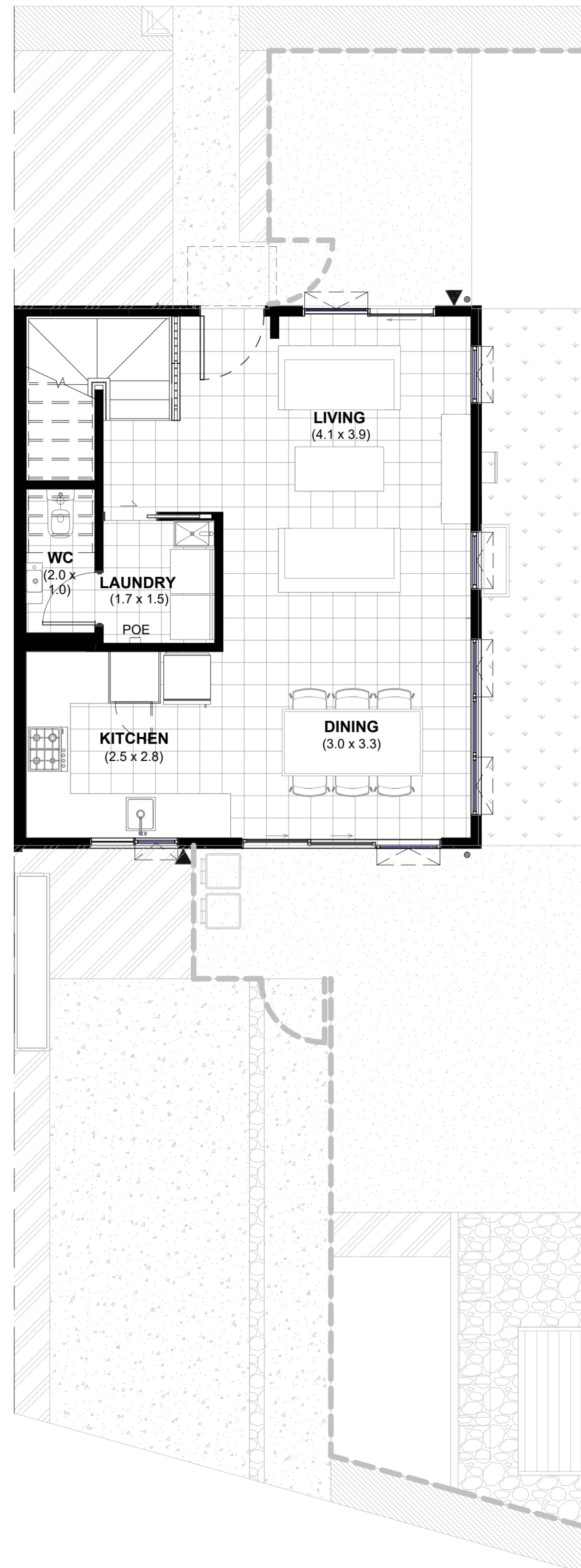
LOT 100 - GROUND FLOOR PLAN
