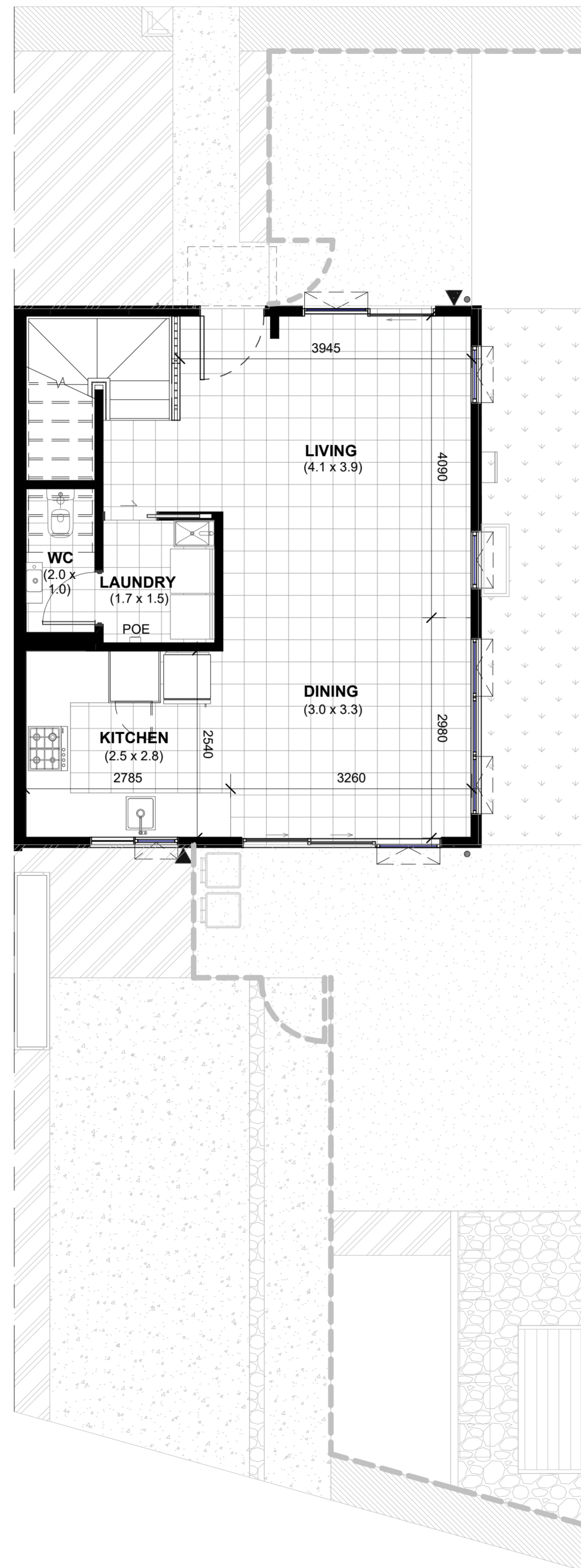
LOT 100 - GROUND FLOOR DIMENSION PLAN
