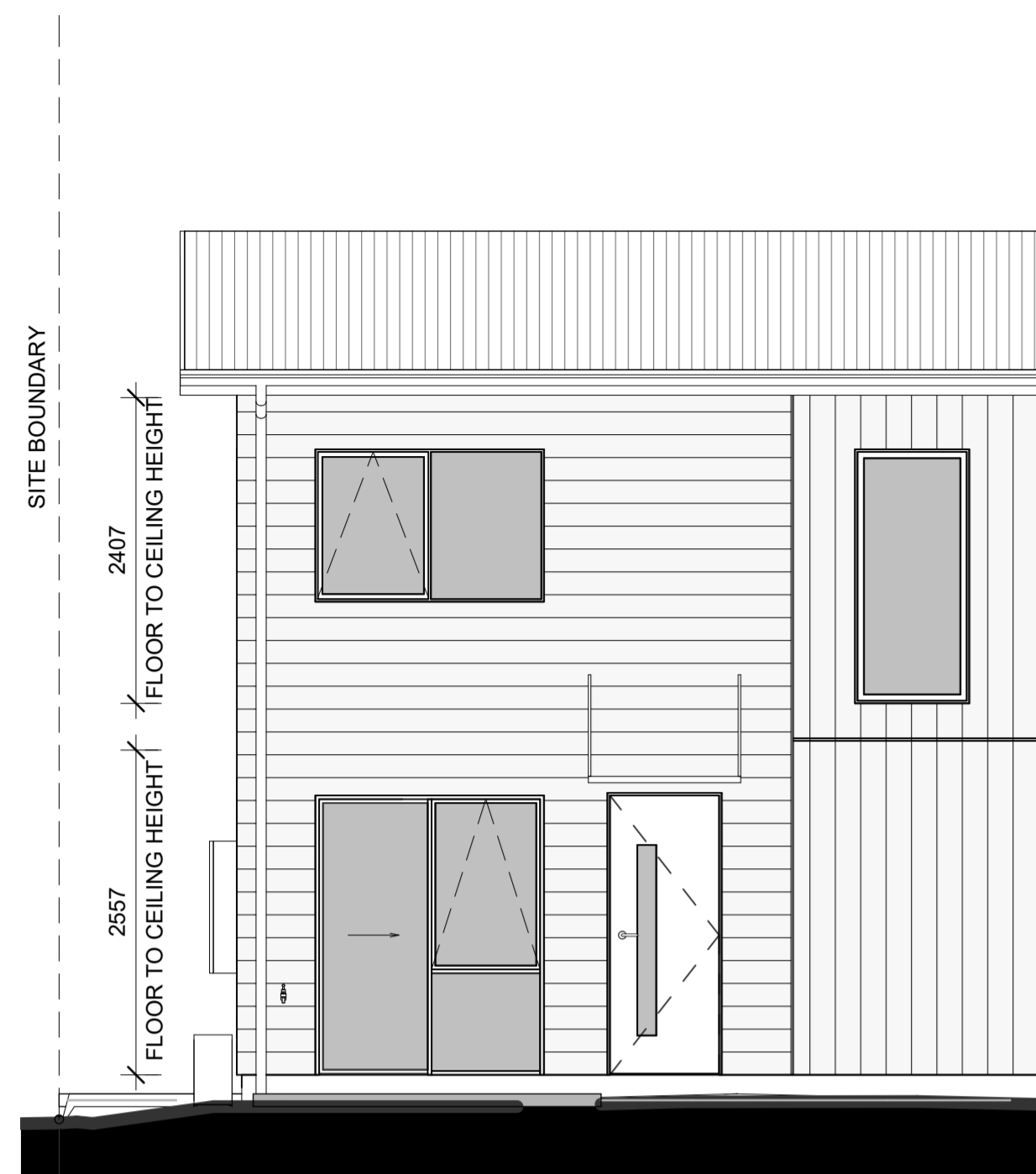
LOT 100 - SOUTH ELEVATION
