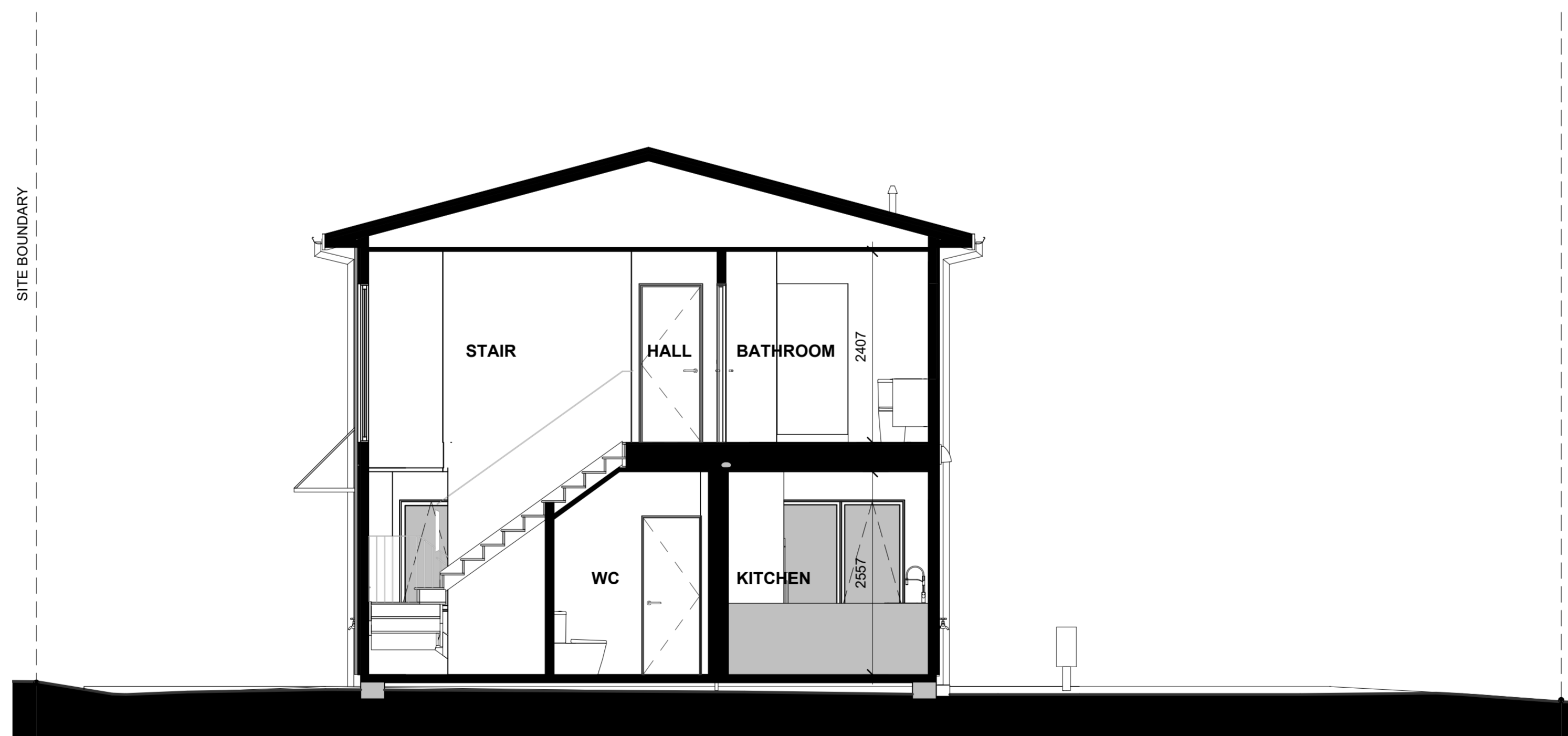
LOT 100 - SECTION A-A
