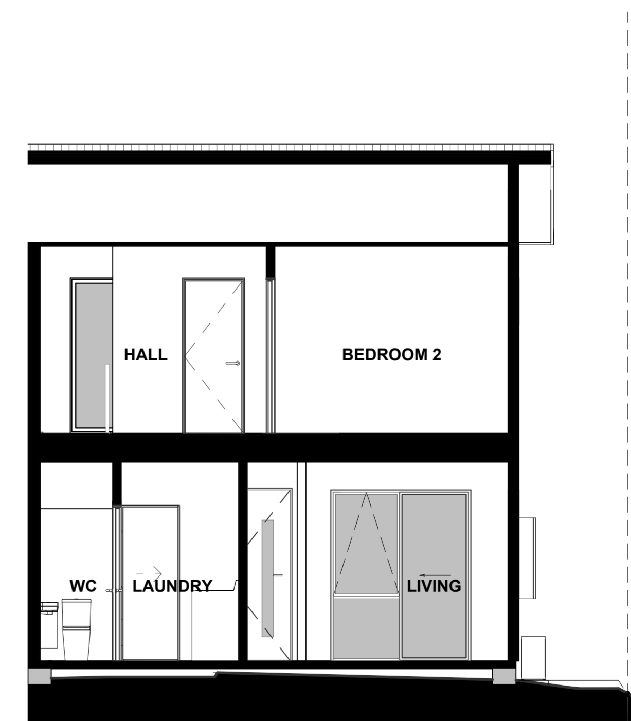
LOT 100 - SECTION B-B
