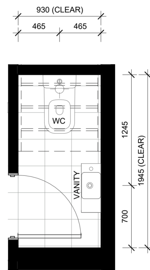
LOT 101 - GROUND FLOOR WC LAYOUT
