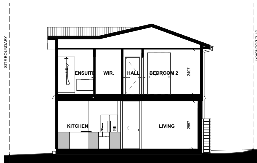
LOT 96 - SECTION C-C
