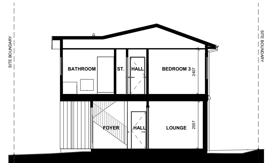
LOT 96 - SECTION B-B
