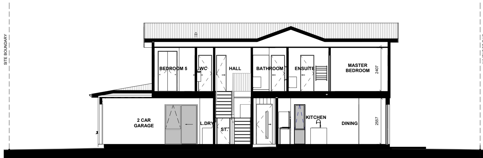
LOT 96 - SECTION A-A
