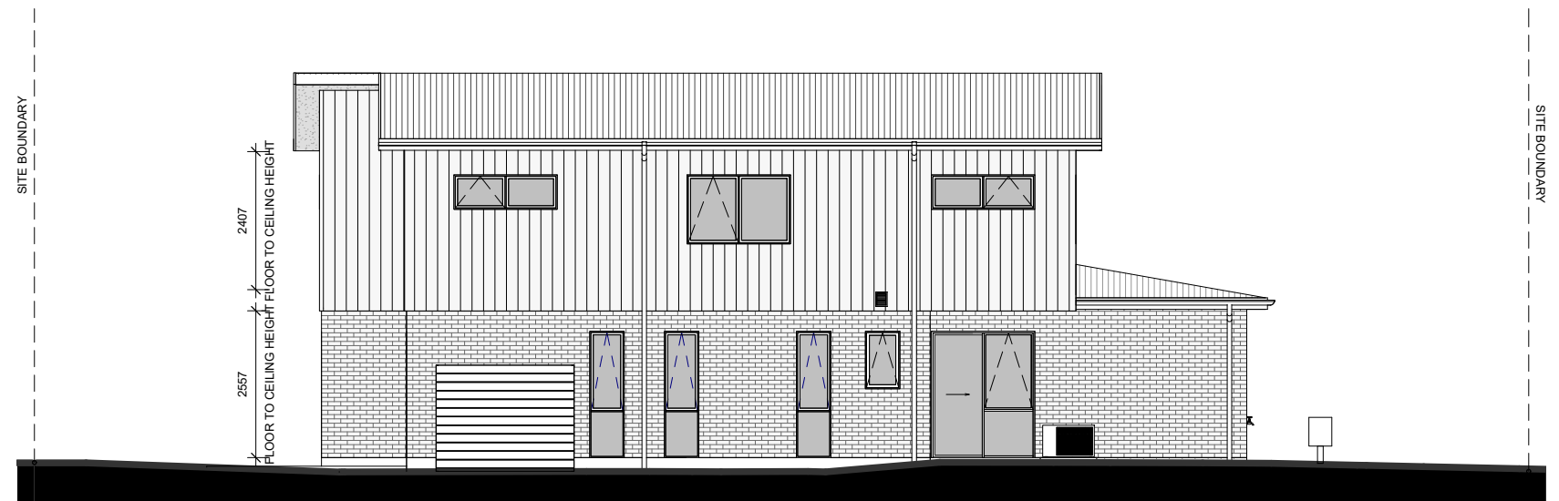
LOT 96 - SOUTH ELEVATION
