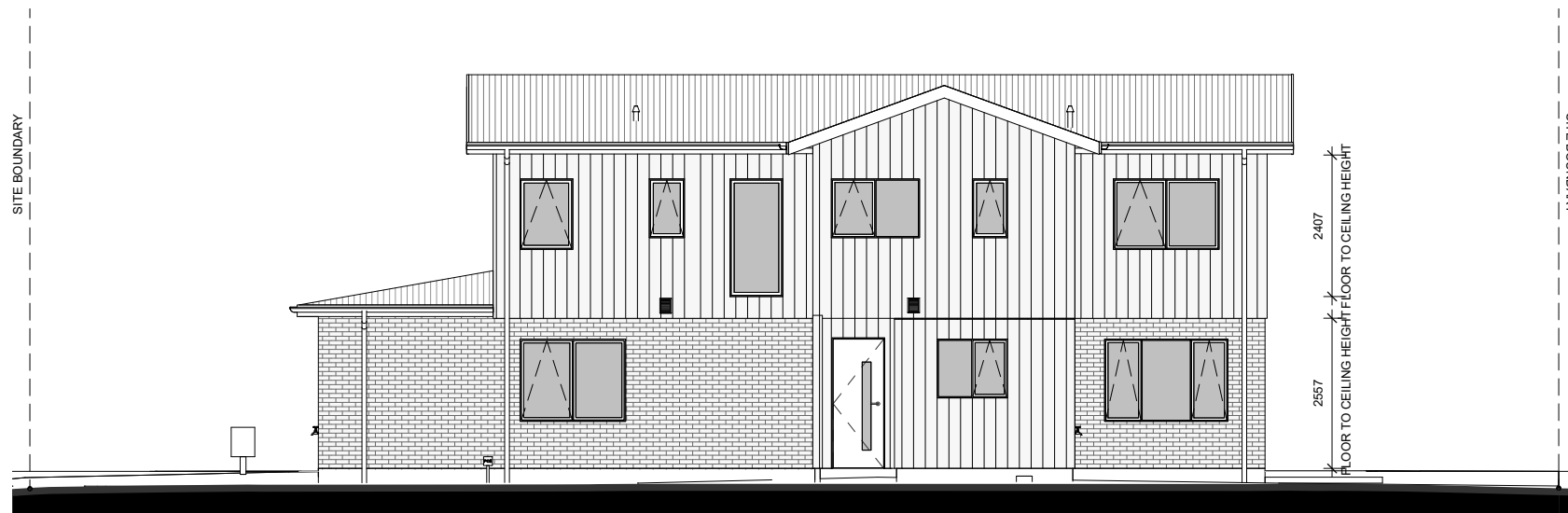
LOT 96 - NORTH ELEVATION
