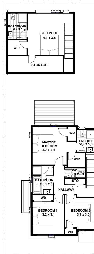
LOT 101 FIRST FLOOR PLAN
