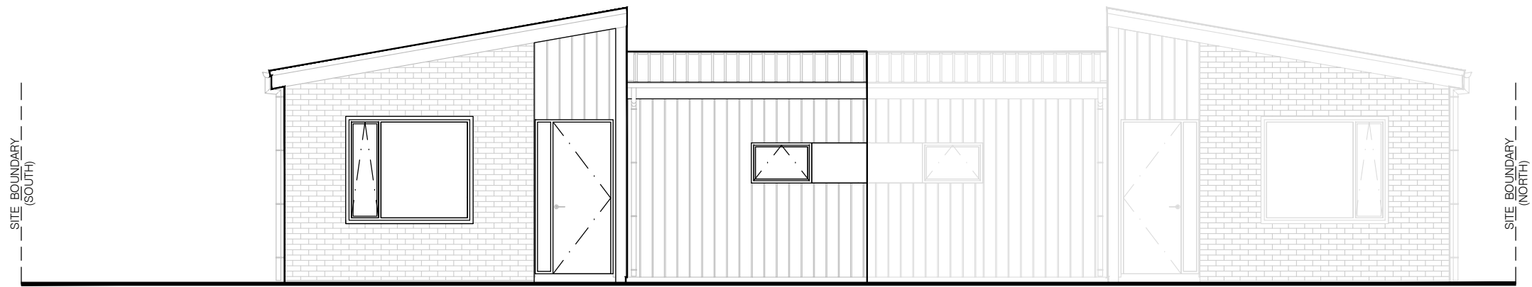
EAST ELEVATION
