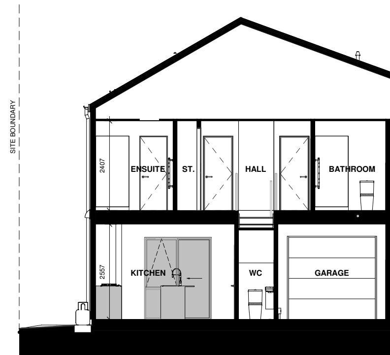
LOT 94 - SECTION B
