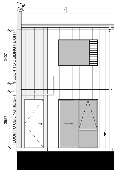
LOT 93 - NORTH ELEVATION
