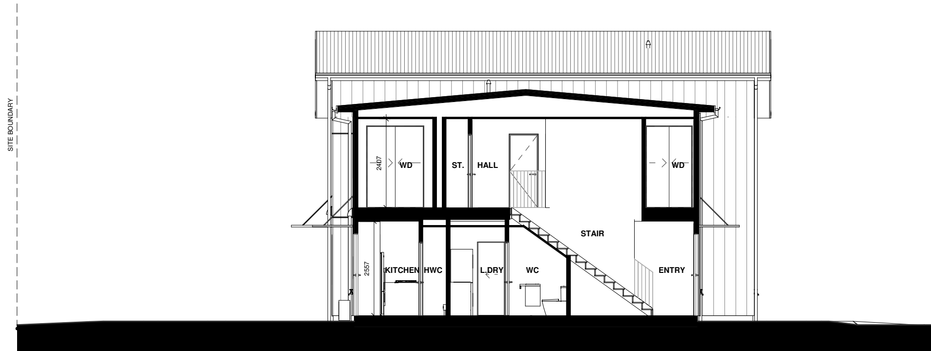
LOT 92 - SECTION A
