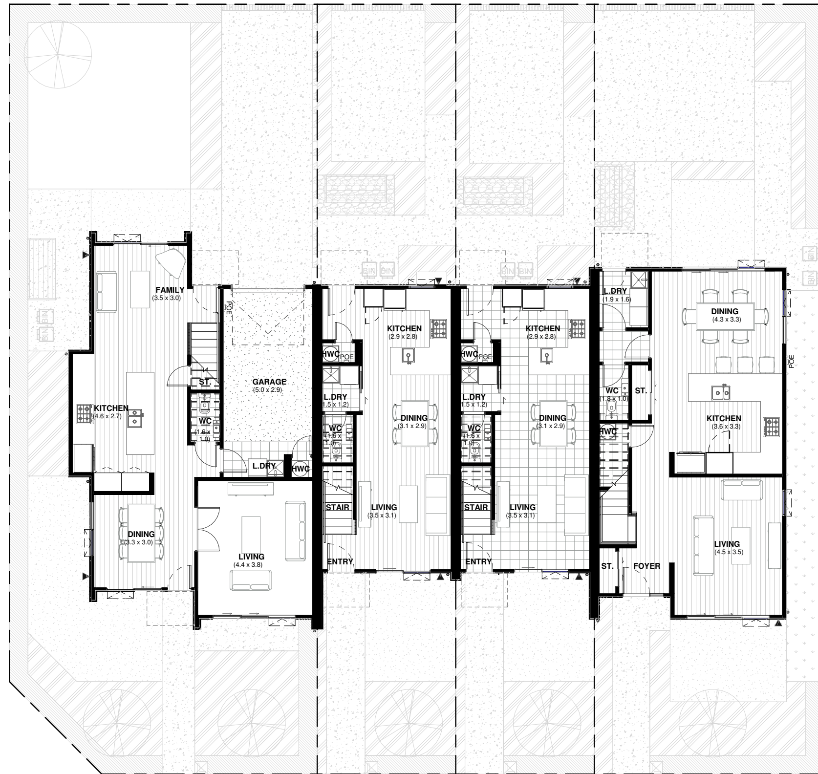
LOT 94 GROUND FLOOR PLAN
