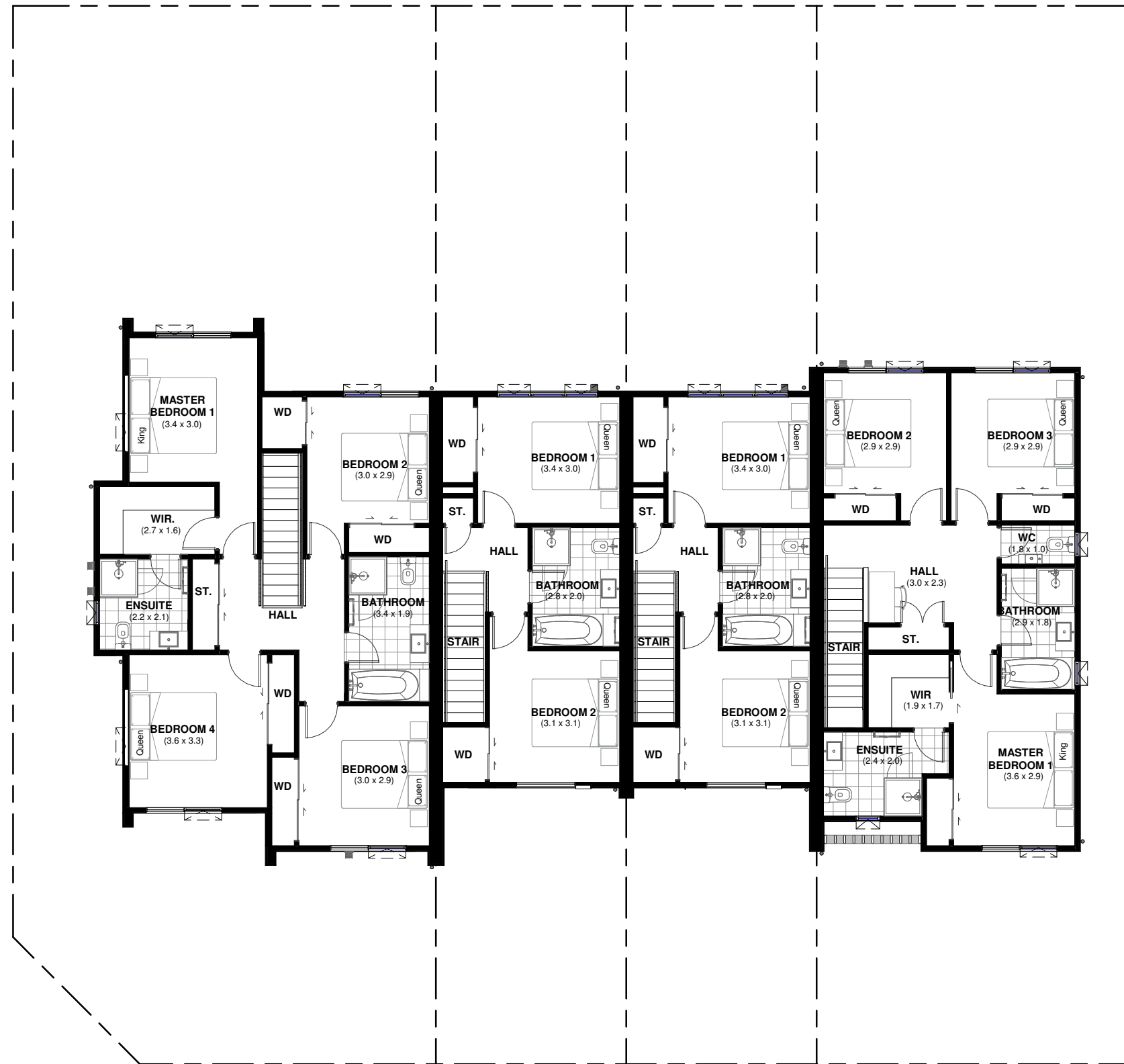
LOT 94 FIRST FLOOR PLAN 2 PORT WAY, HINGAIA Floor Area - 166m 2 Site Area - 246m 2 Ground Floor - 82m 2 First Floor - 83m 2
