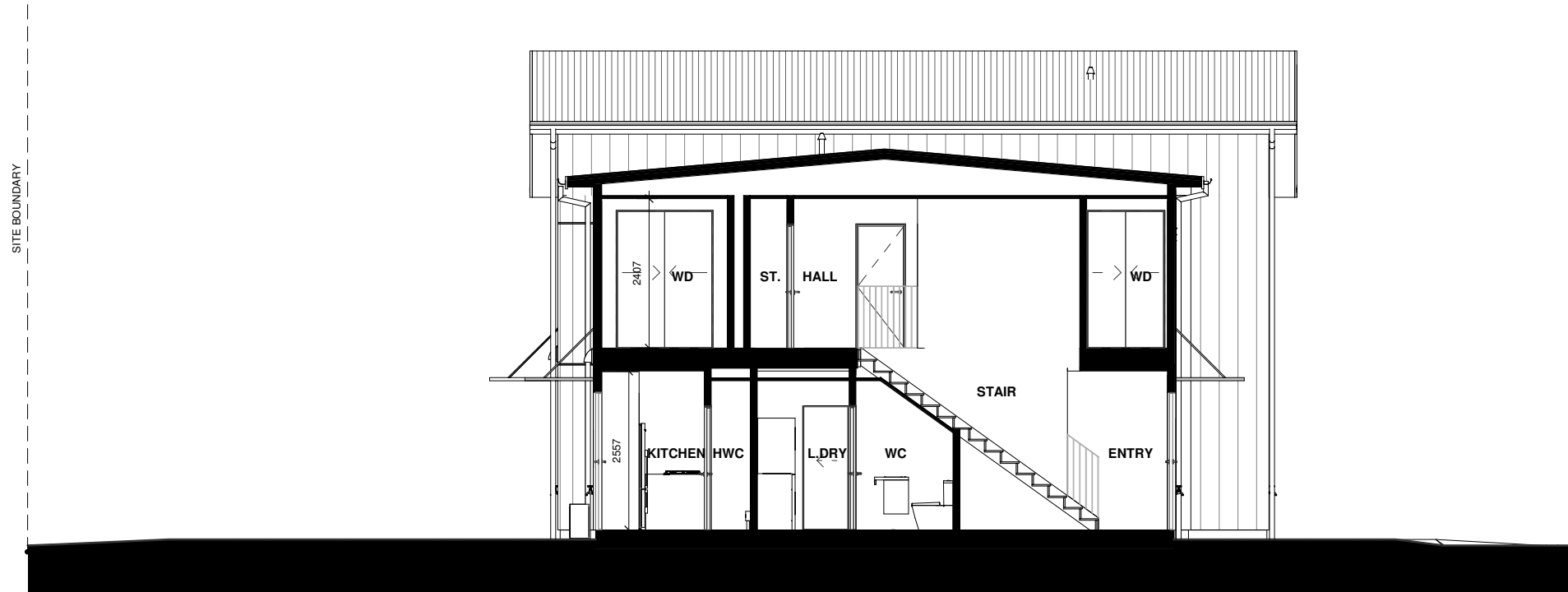
LOT 93 - SECTION A
