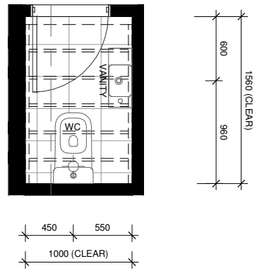
LOT 93 - GROUND FLOOR WC LAYOUT
