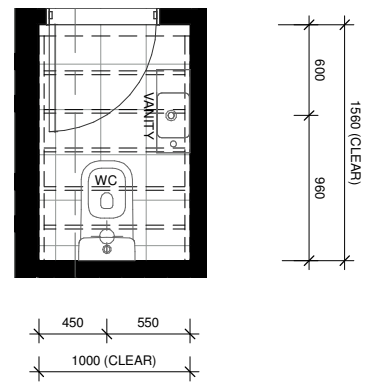
LOT 92 - GROUND FLOOR WC LAYOUT
