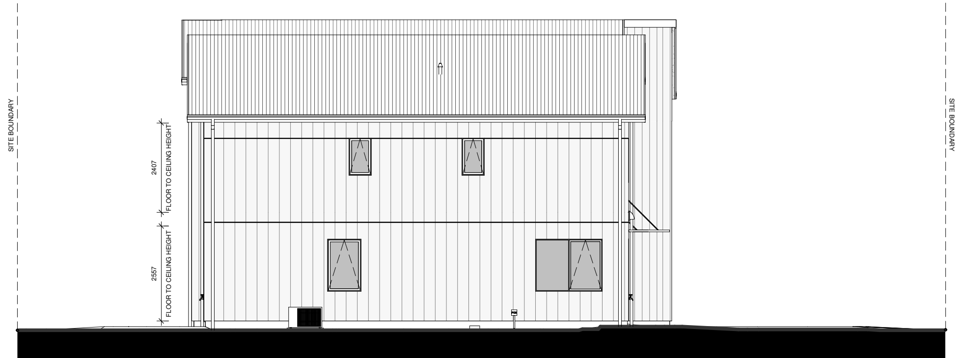
LOT 91 - WEST ELEVATION
