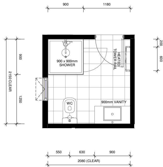
LOT 94 - FIRST FLOOR ENSUITE LAYOUT
