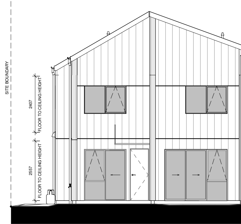
LOT 94 - NORTH ELEVATION
