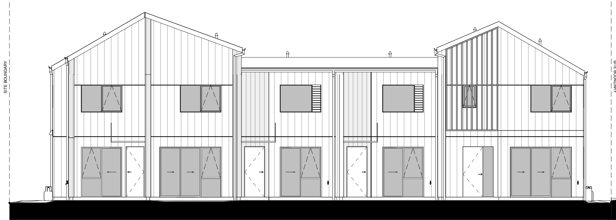
OVERALL NORTH ELEVATION
