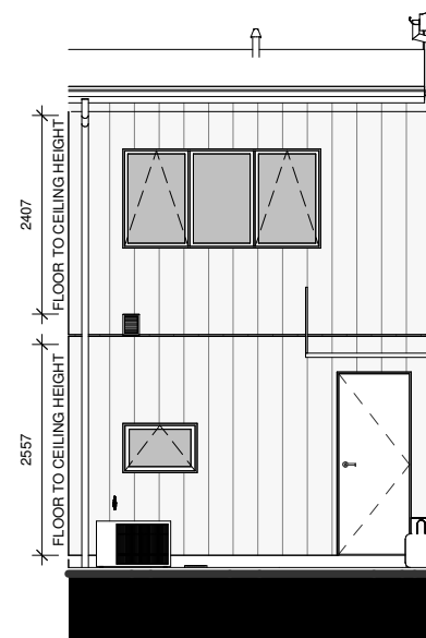
LOT 93 - SOUTH ELEVATION
