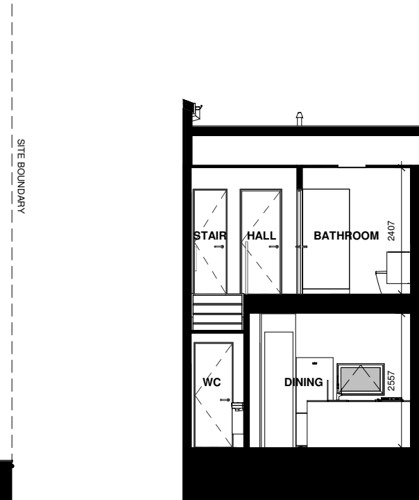
LOT 93 - SECTION B
