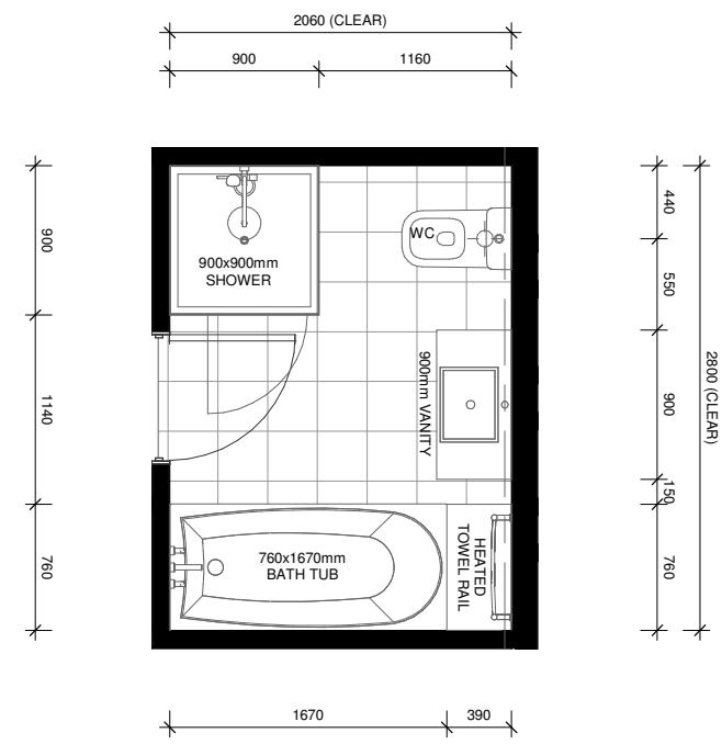
LOT 92 - FIRST FLOOR BATHROOM LAYOUT
