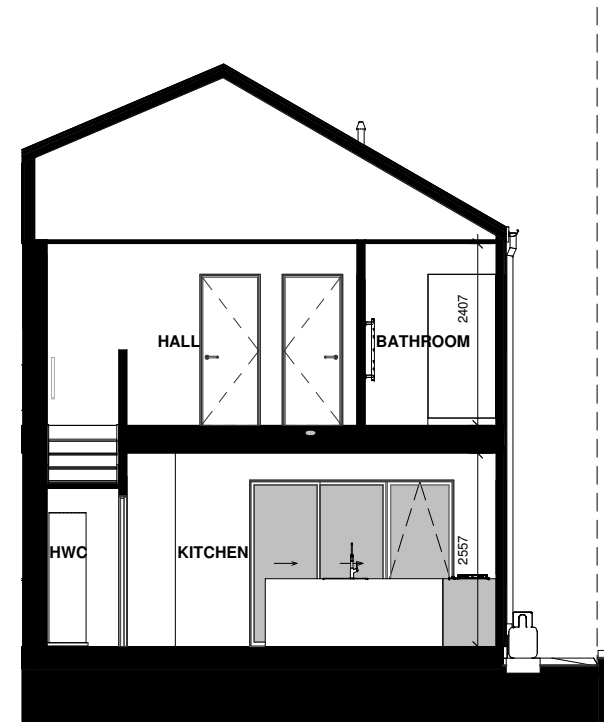
LOT 91 - SECTION B
