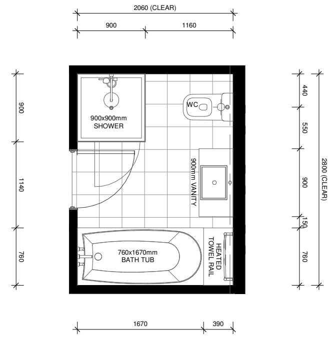
LOT 93 - FIRST FLOOR BATHROOM LAYOUT
