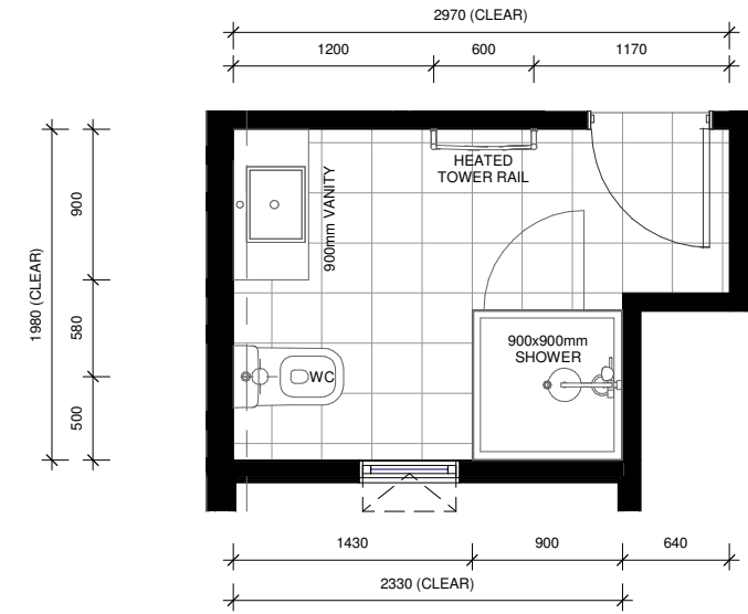
LOT 91 - FIRST FLOOR ENSUITE LAYOUT
