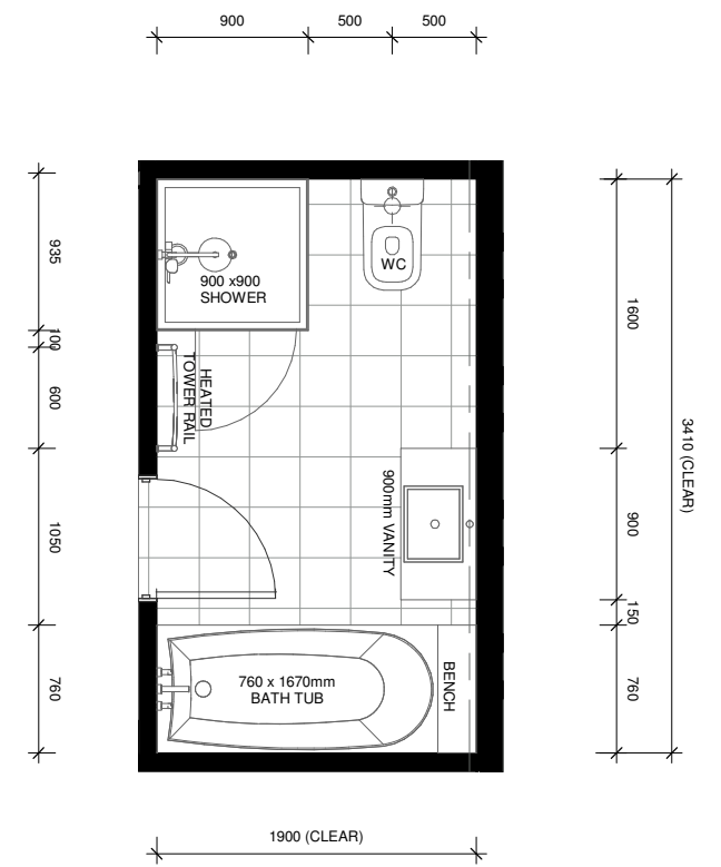
LOT 94 - FIRST FLOOR BATHROOM LAYOUT
