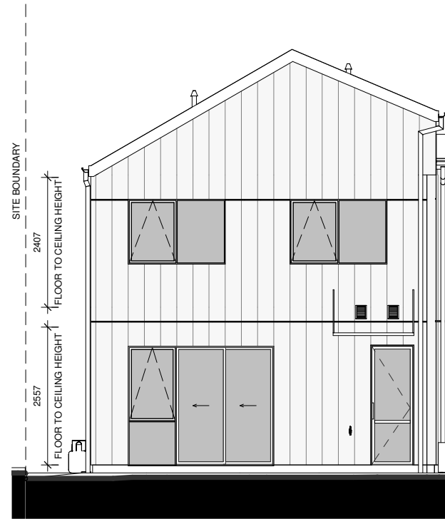
LOT 91 - SOUTH ELEVATION
