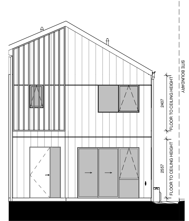
LOT 91 - NORTH ELEVATION
