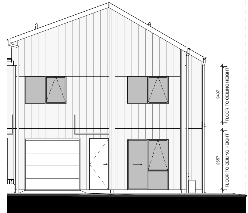
LOT 94 - SOUTH ELEVATION
