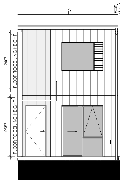
LOT 92 - NORTH ELEVATION
