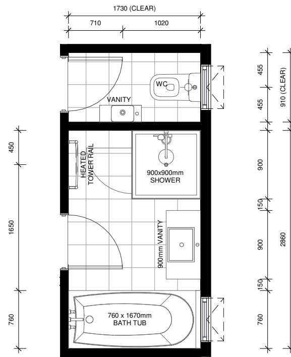
LOT 91 - FIRST FLOOR BATHROOM & WC LAYOUT
